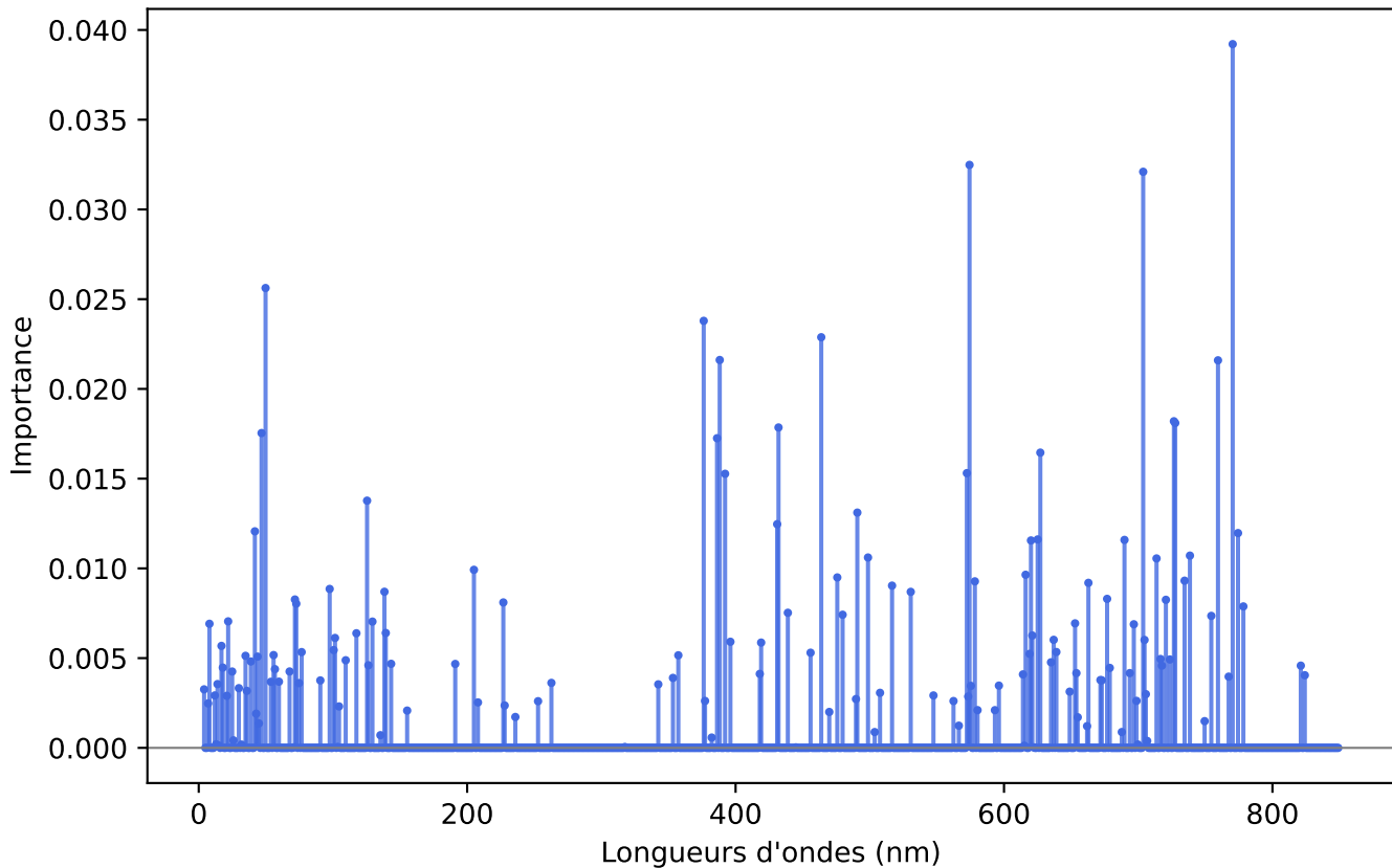
XGB Importance Variables (Iter 1)
