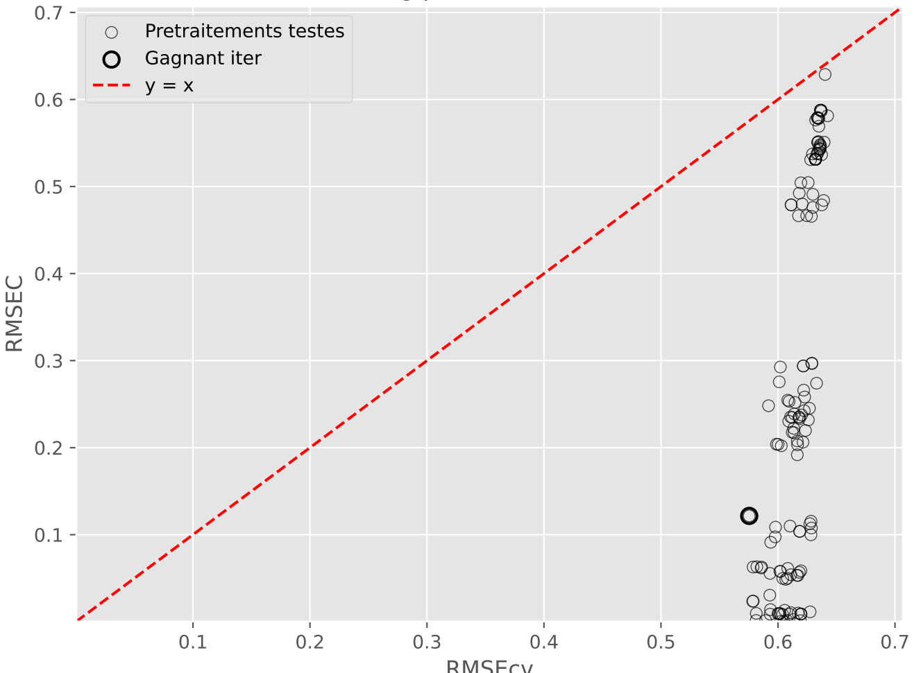
Overfitting pretraitements (Iter 2)
