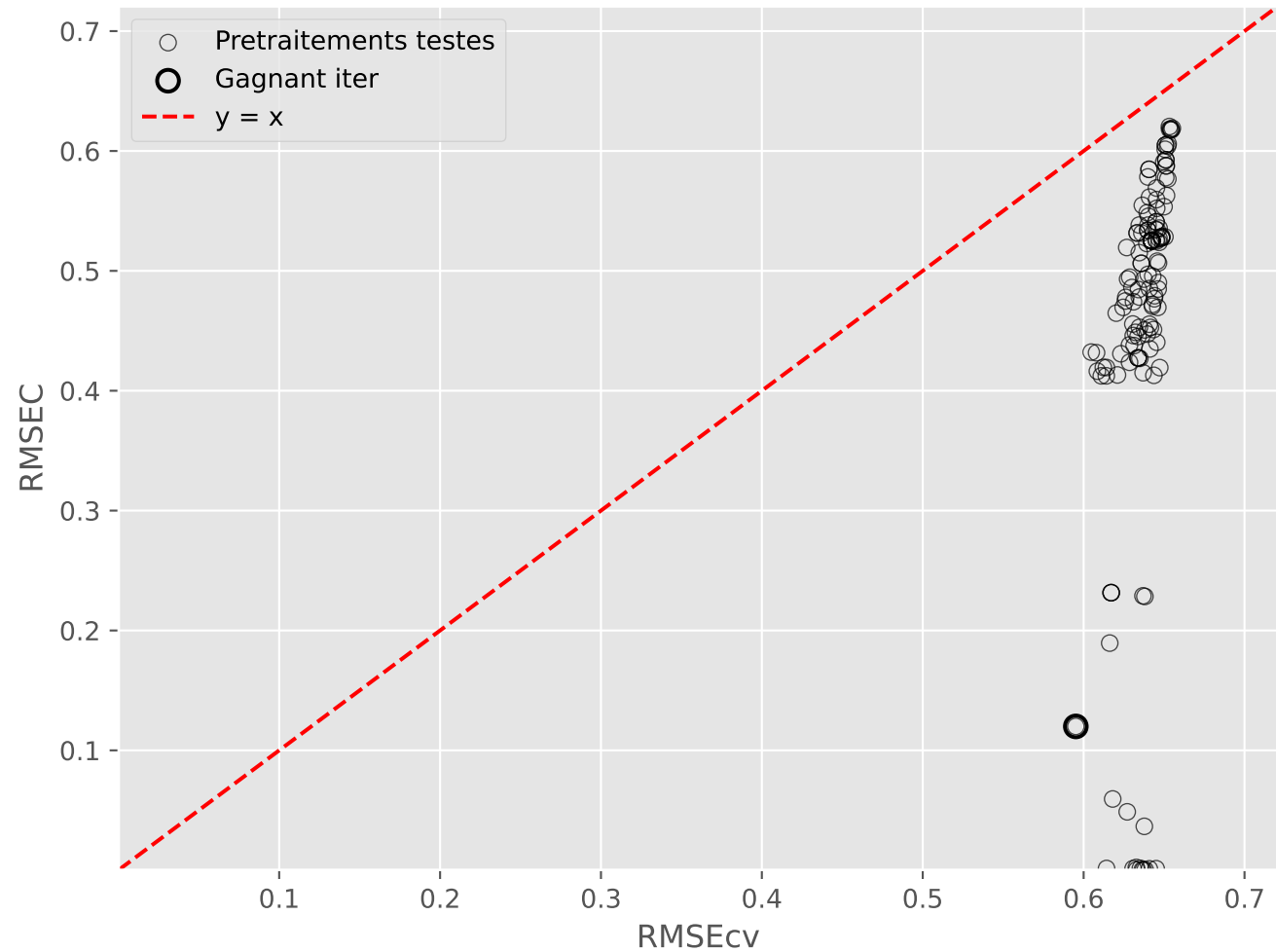
Overfitting pretraitements (Iter 6)
