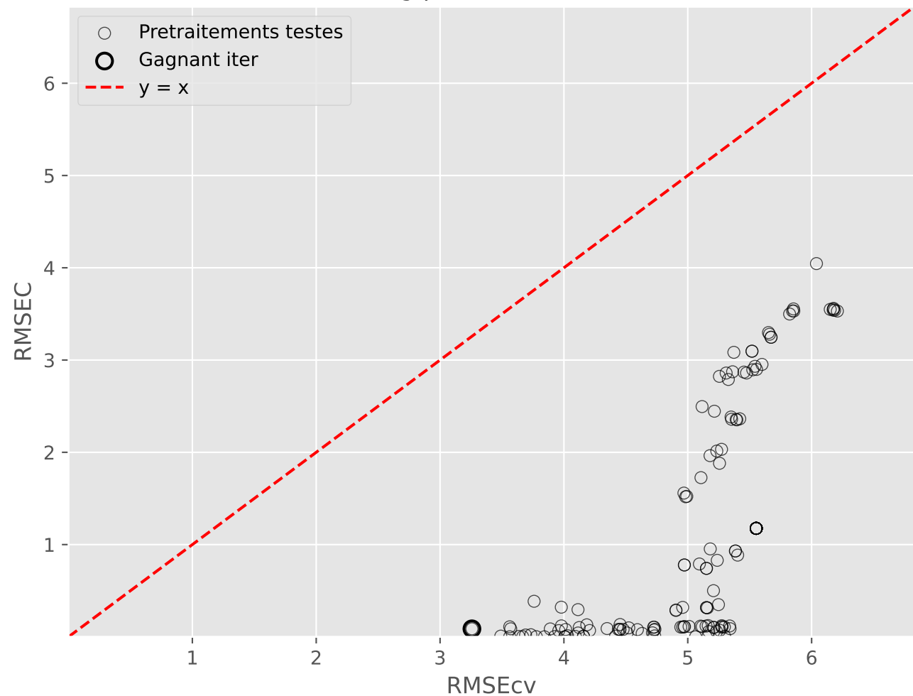
Overfitting pretraitements (Iter 7)
