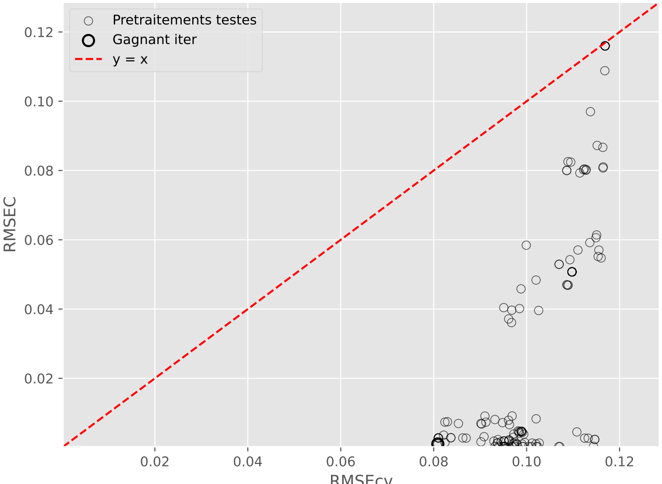
Overfitting pretraitements (Iter 5)
