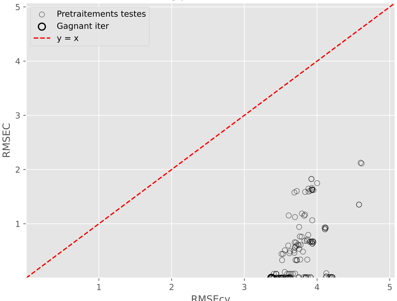
Overfitting pretraitements (Iter 9)
