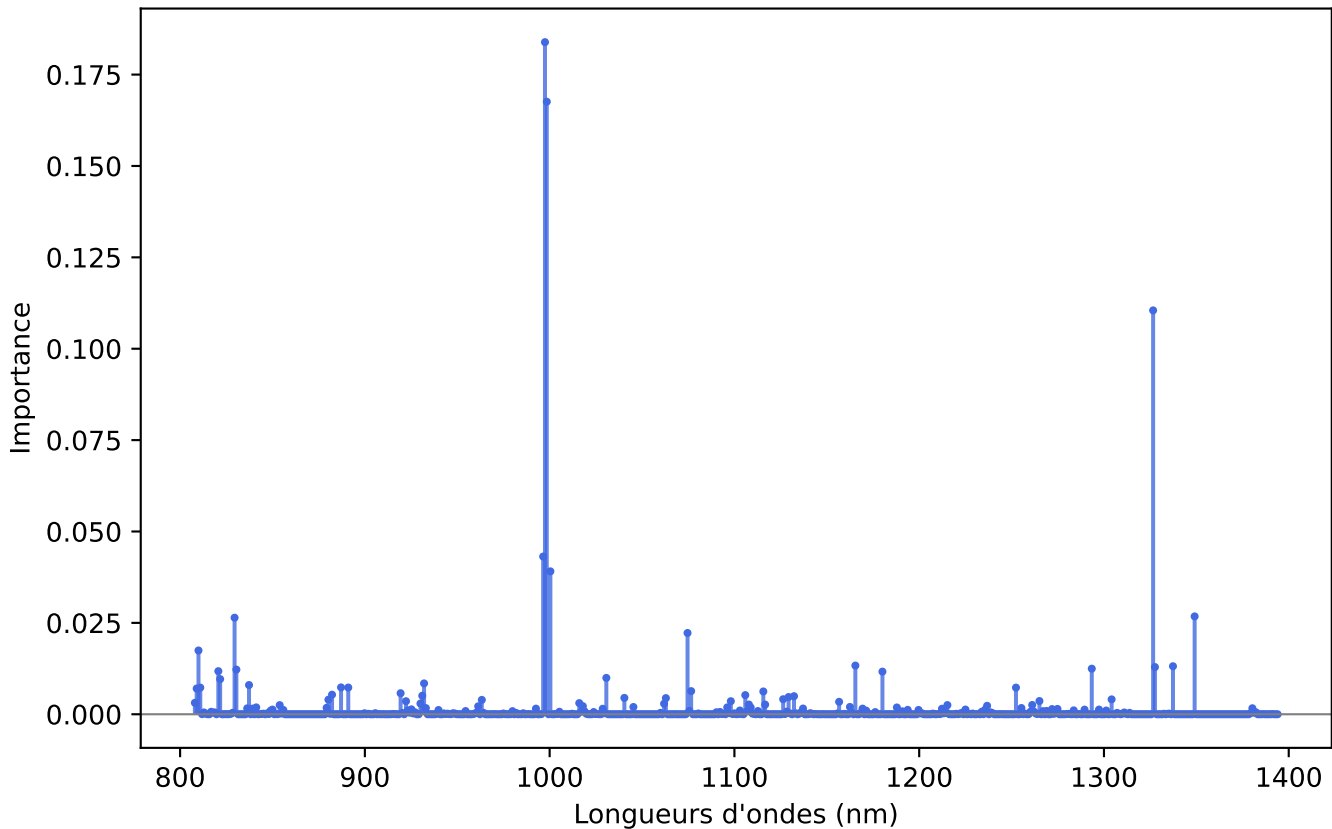
XGB Importance Variables (Iter 9)
