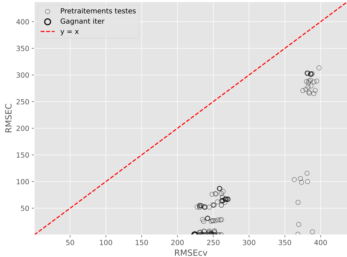
Overfitting pretraitements (Iter 9)
