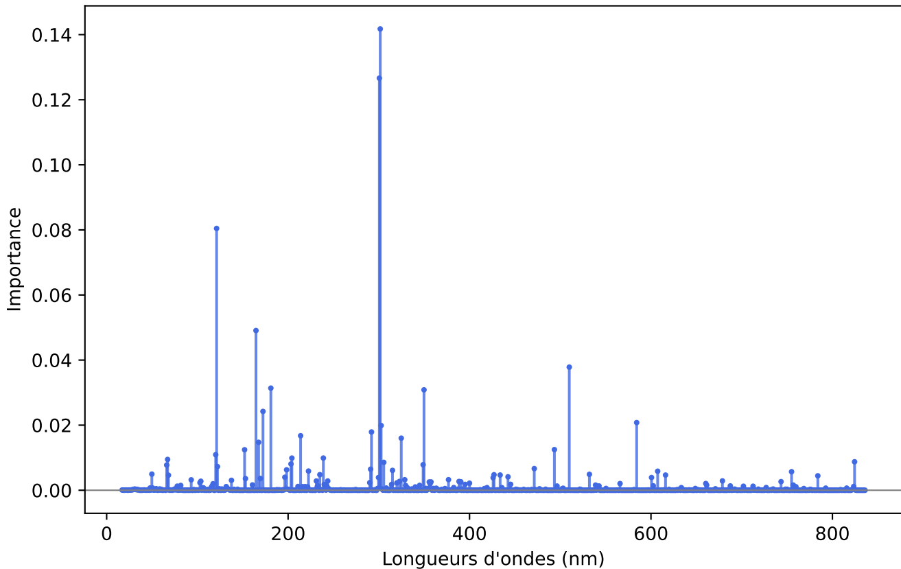
XGB Importance Variables (Iter 9)
