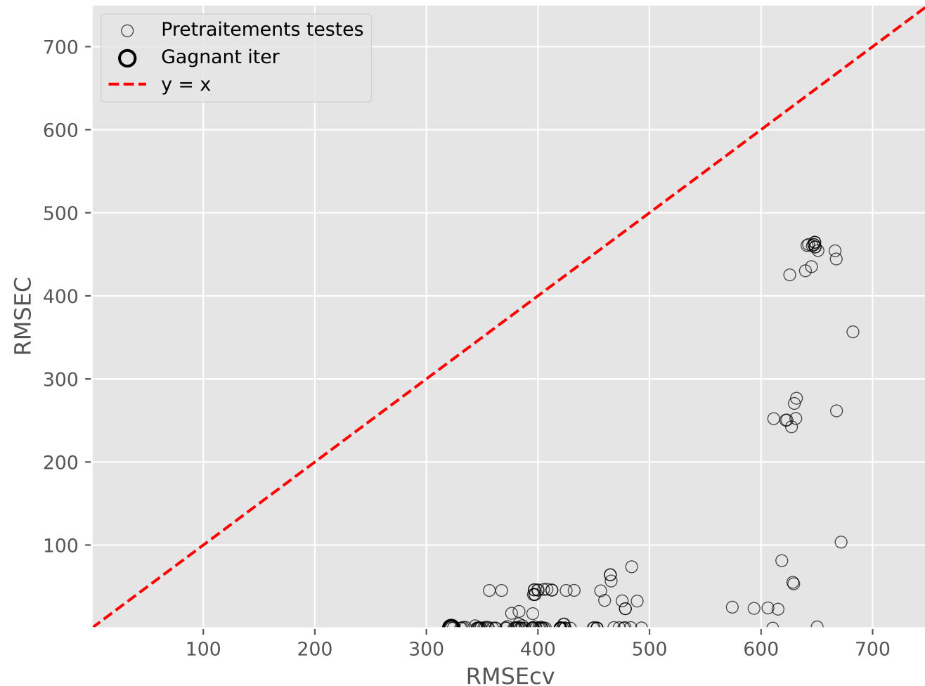
Overfitting pretraitements (Iter 7)
