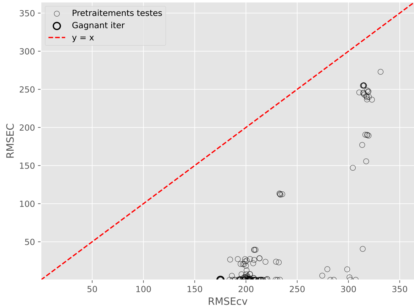
Overfitting pretraitements (Iter 10)
