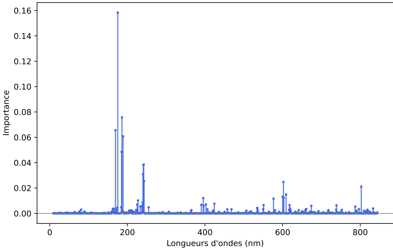
XGB Importance Variables (Iter 10)
