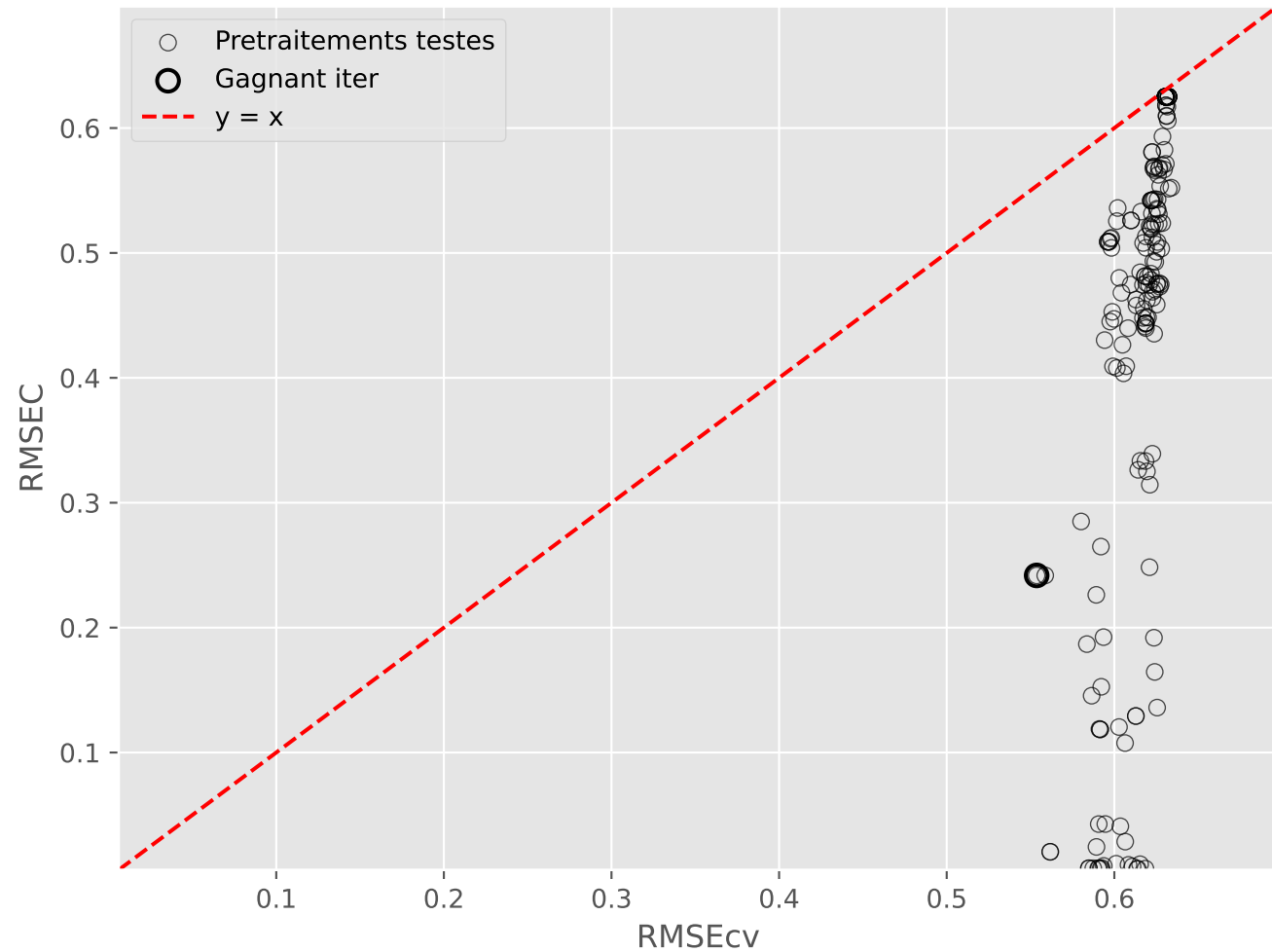
Overfitting pretraitements (Iter 4)
