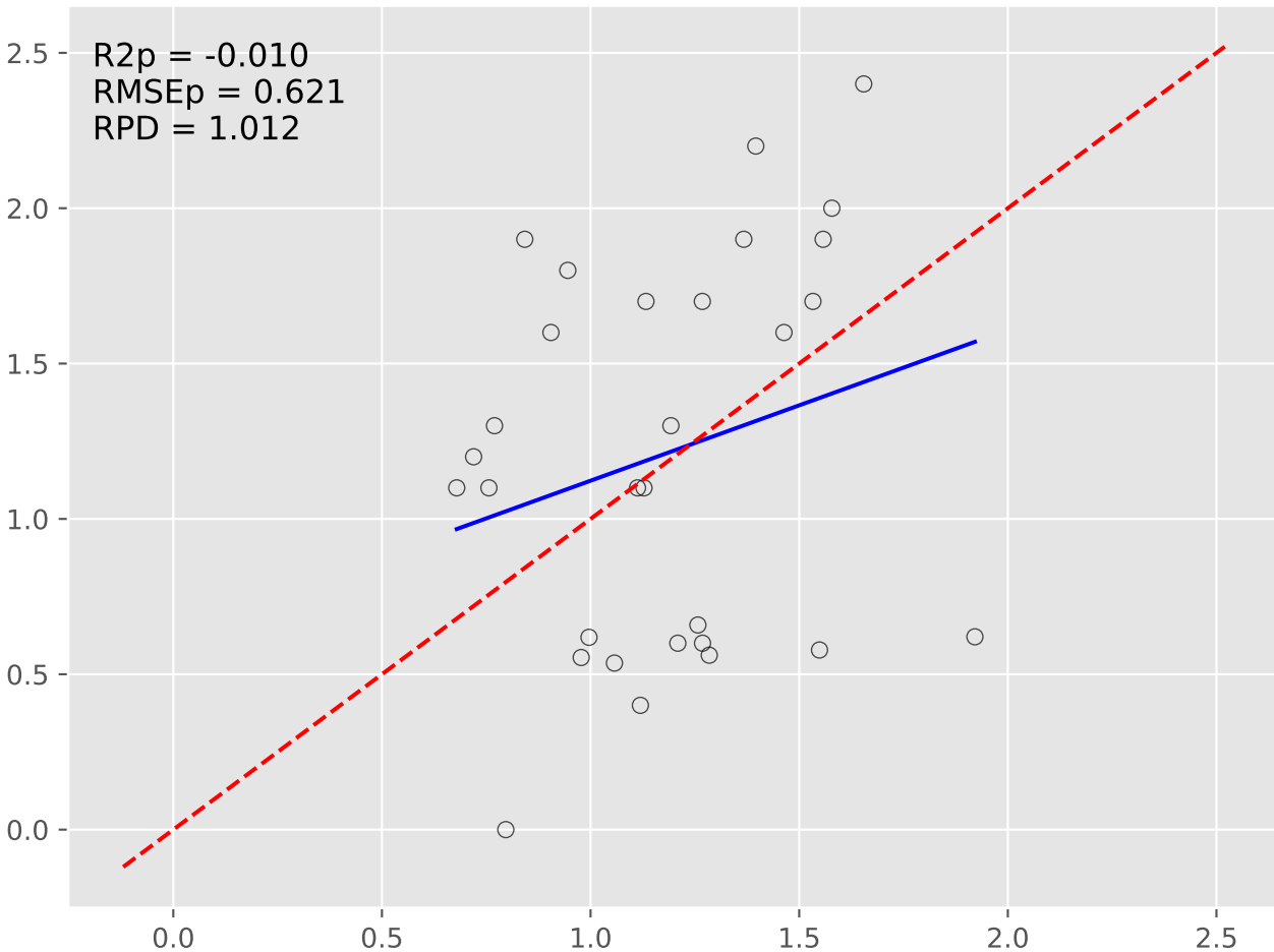
Predictions vs Mesures (Iter 9)
