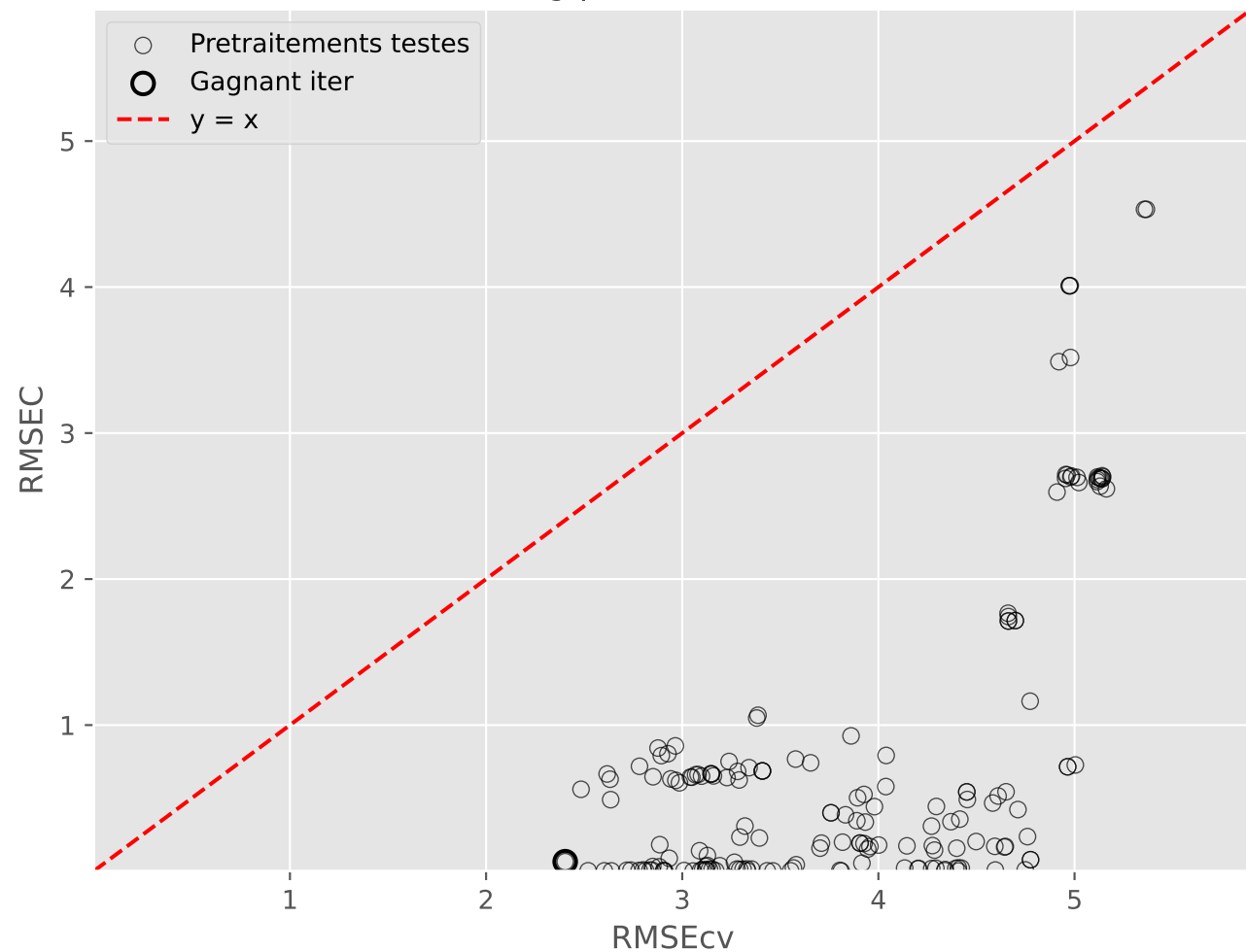
Overfitting pretraitements (Iter 6)
