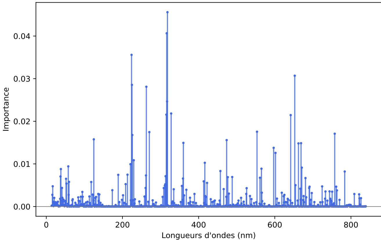
XGB Importance Variables (Iter 3)
