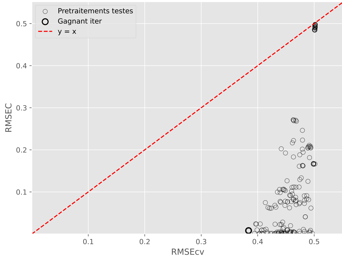
Overfitting pretraitements (Iter 3)
