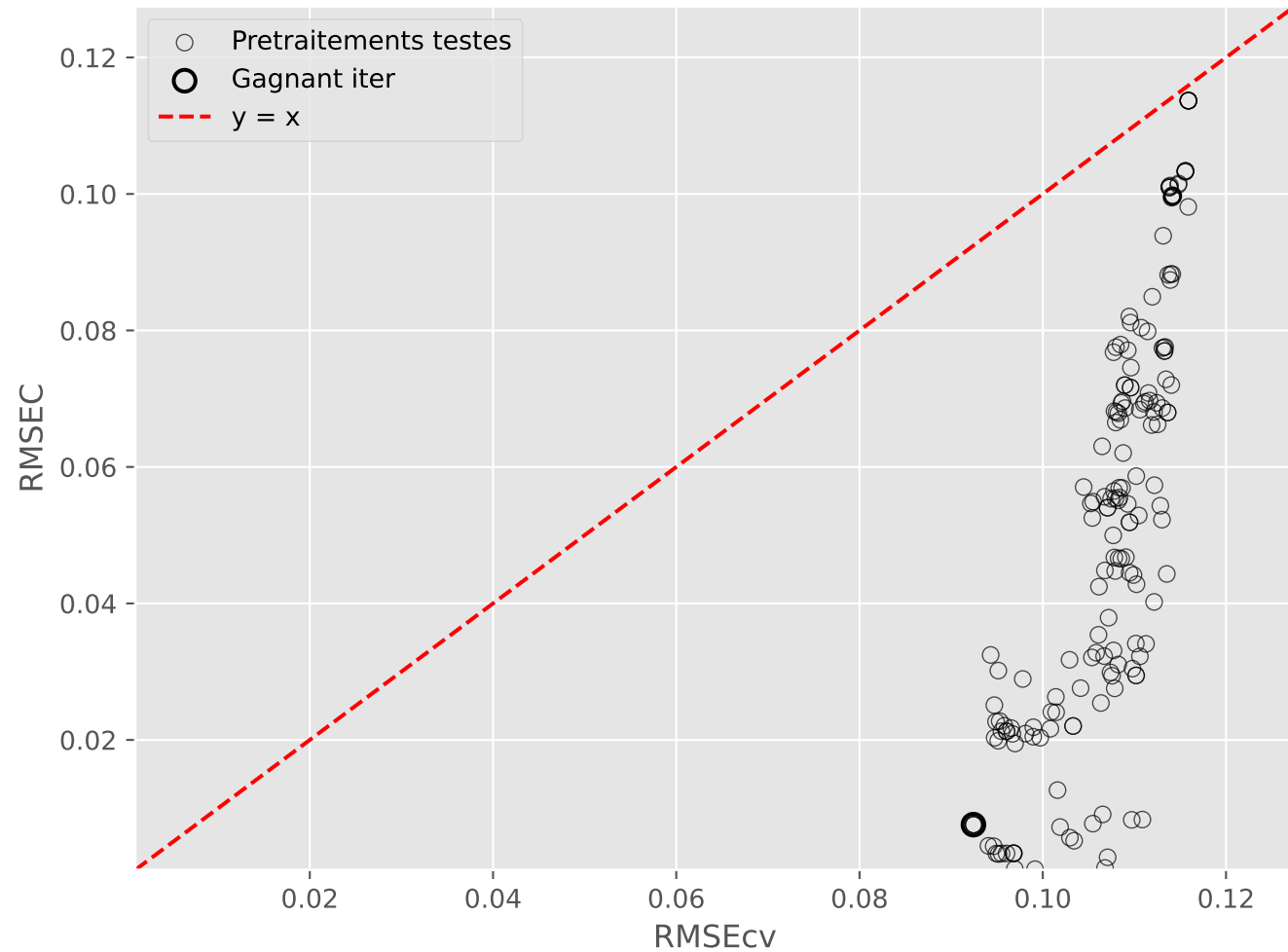
Overfitting pretraitements (Iter 8)
