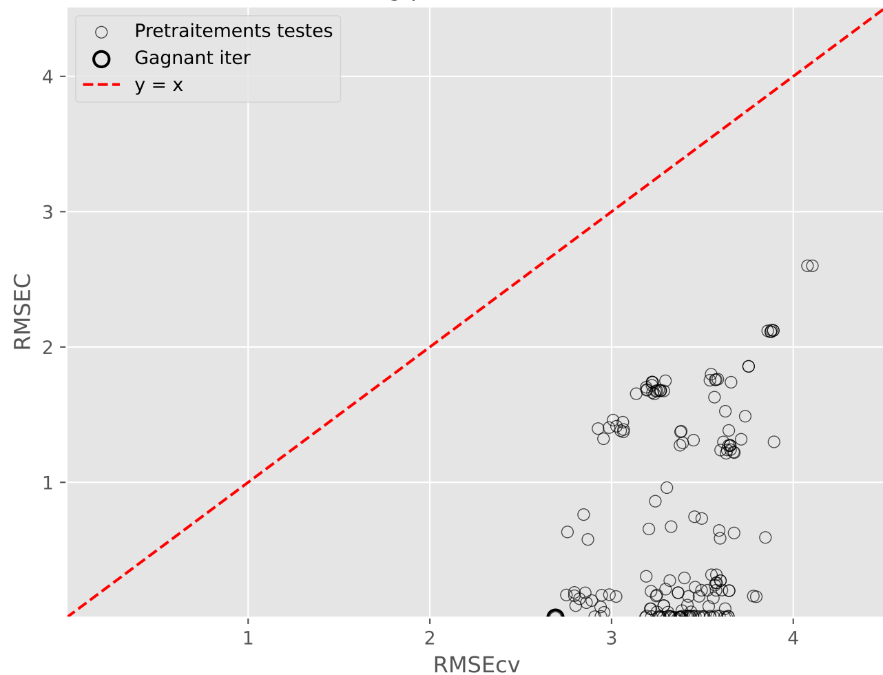
Overfitting pretraitements (Iter 1)
