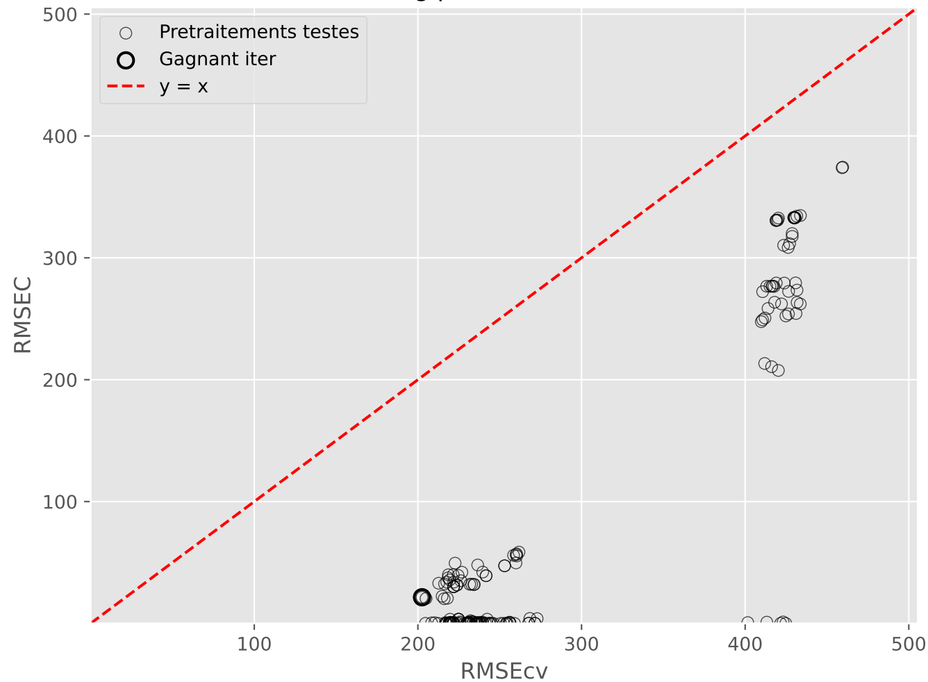
Overfitting pretraitements (Iter 7)
