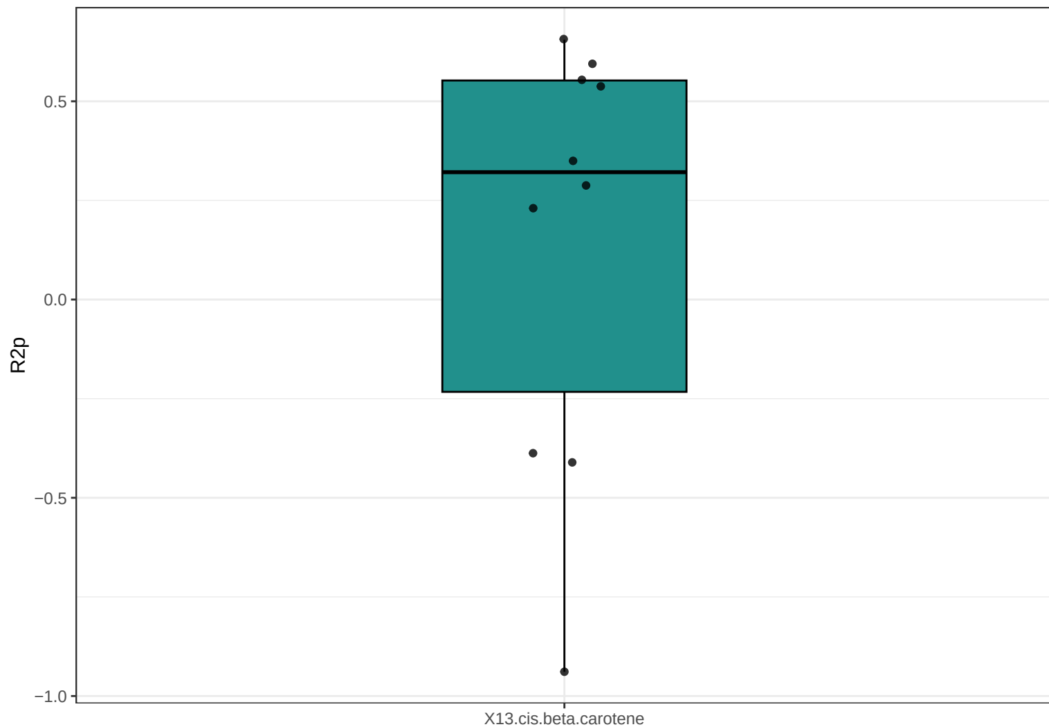
Boxplot R2p (PLS) : X13.cis.beta.carotene
