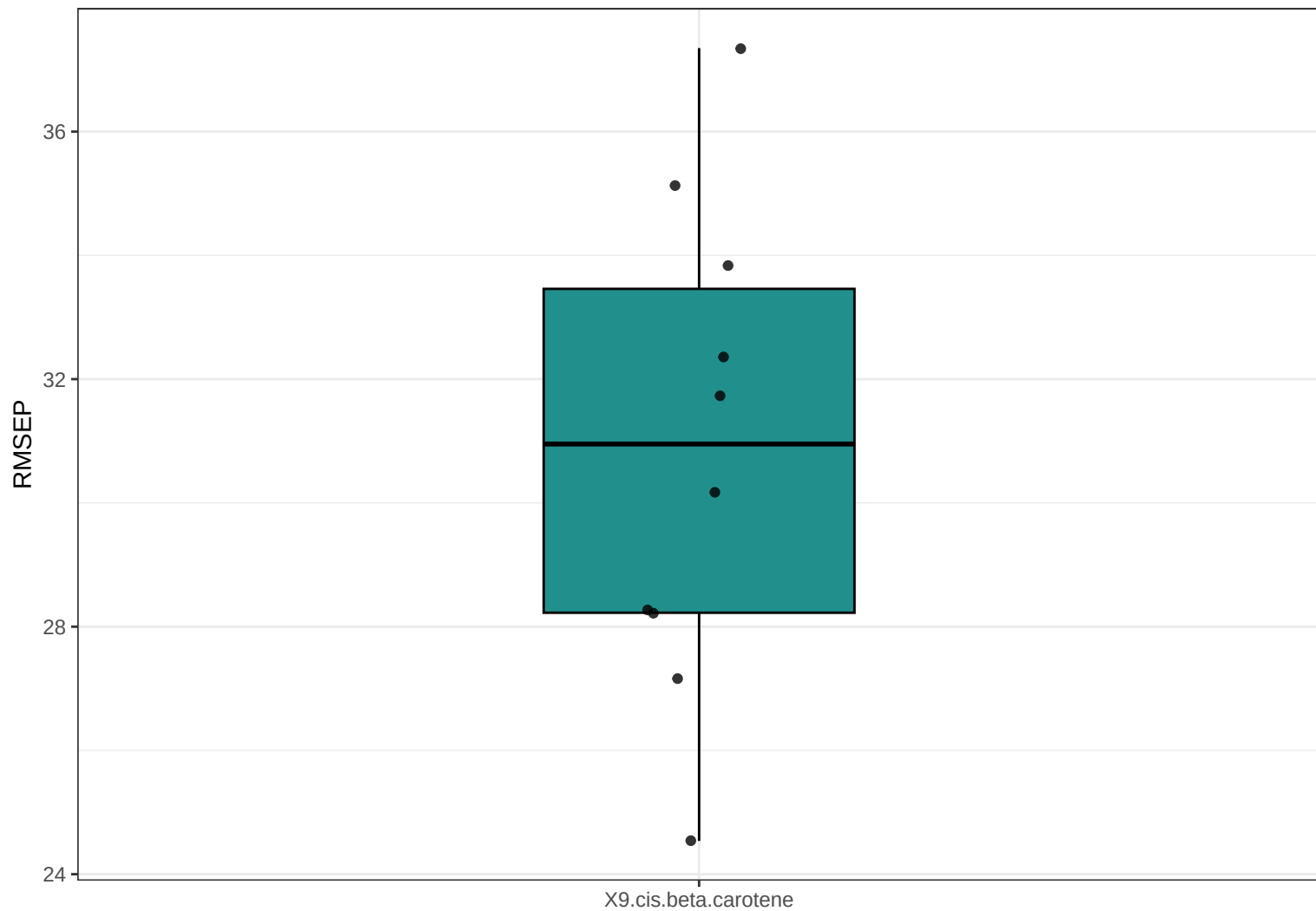
Boxplot RMSEP (PLS) : X9.cis.beta.carotene
