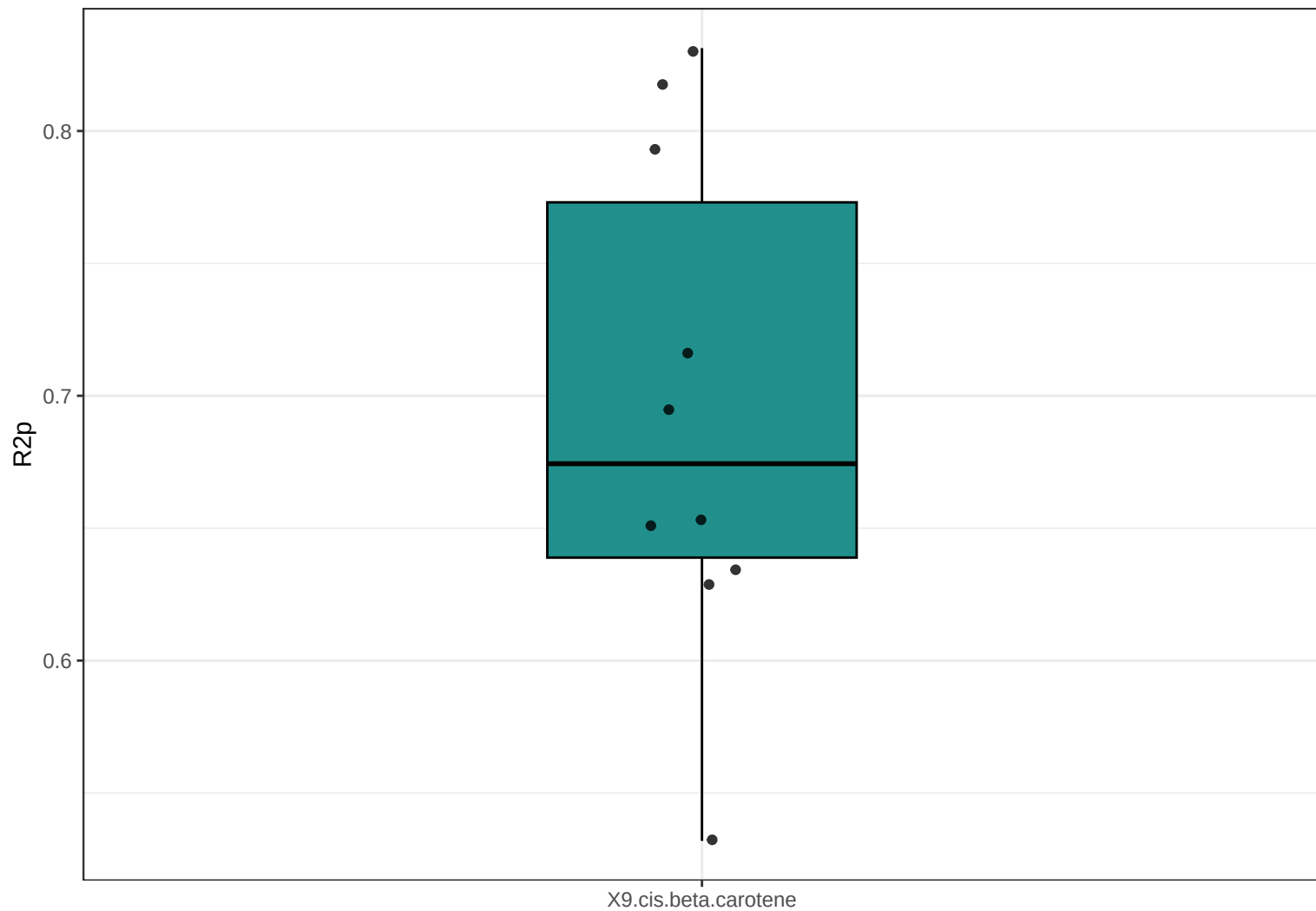
Boxplot R2p (PLS) : X9.cis.beta.carotene
