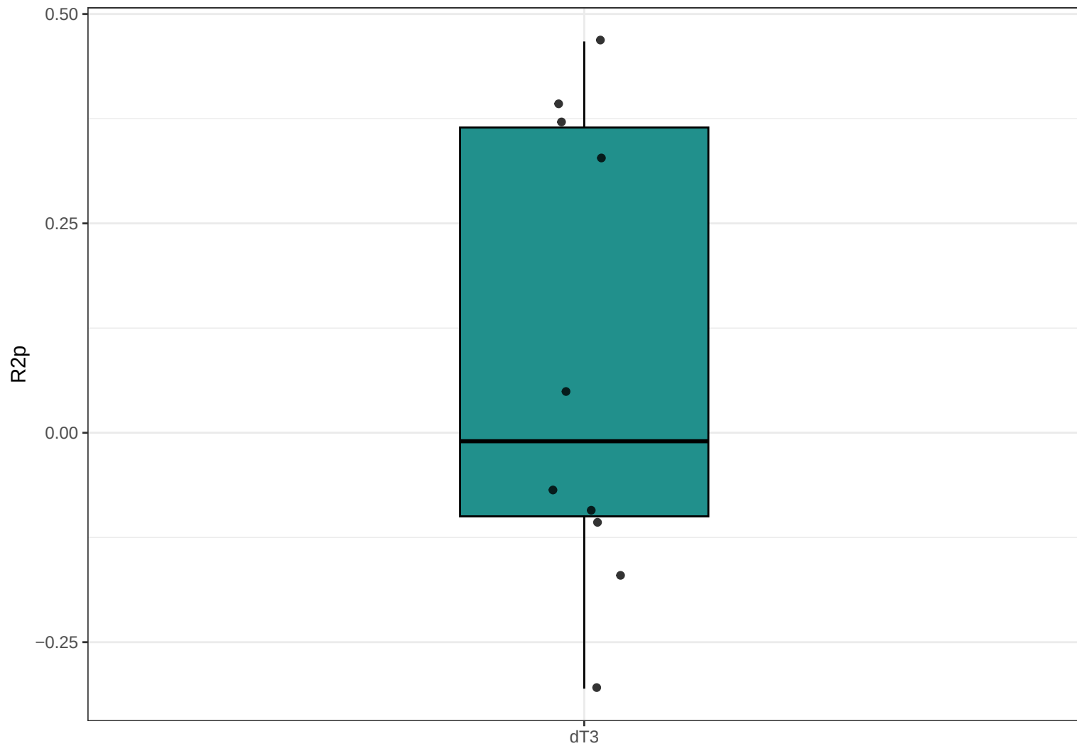
Boxplot R2p (PLS) : dT3
