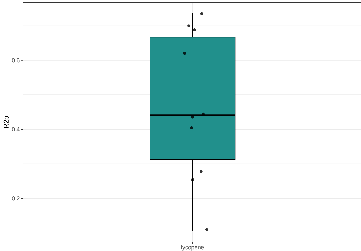
Boxplot R2p (PLS) : lycopene
