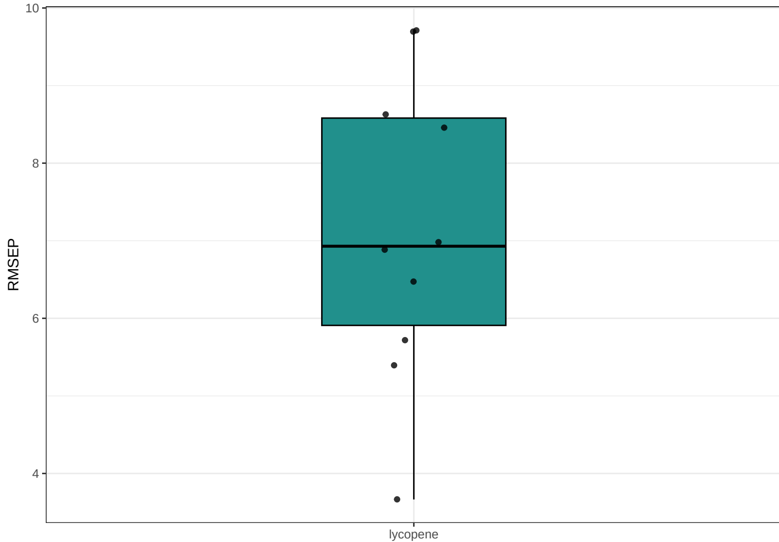
Boxplot RMSEP (PLS) : lycopene
