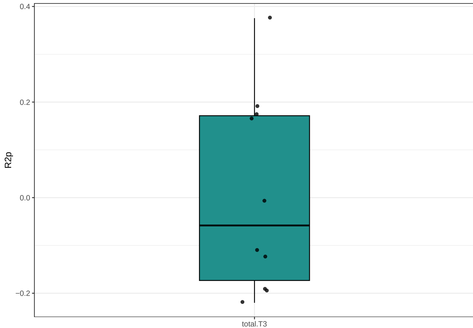
Boxplot R2p (PLS) : total.T3
