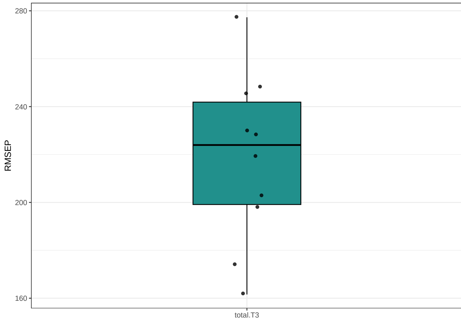
Boxplot RMSEP (PLS) : total.T3
