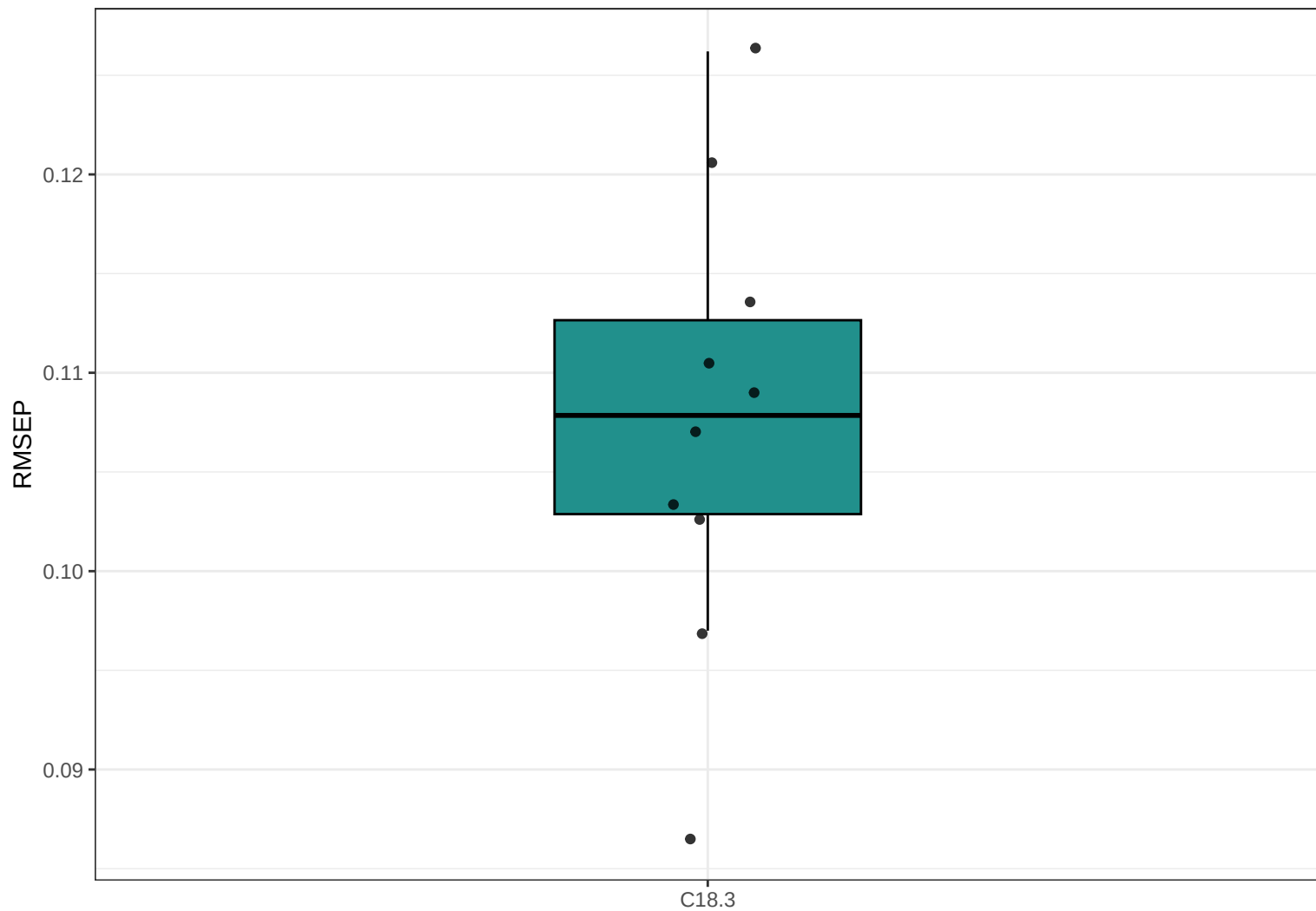
Boxplot RMSEP (PLS) : C18.3
