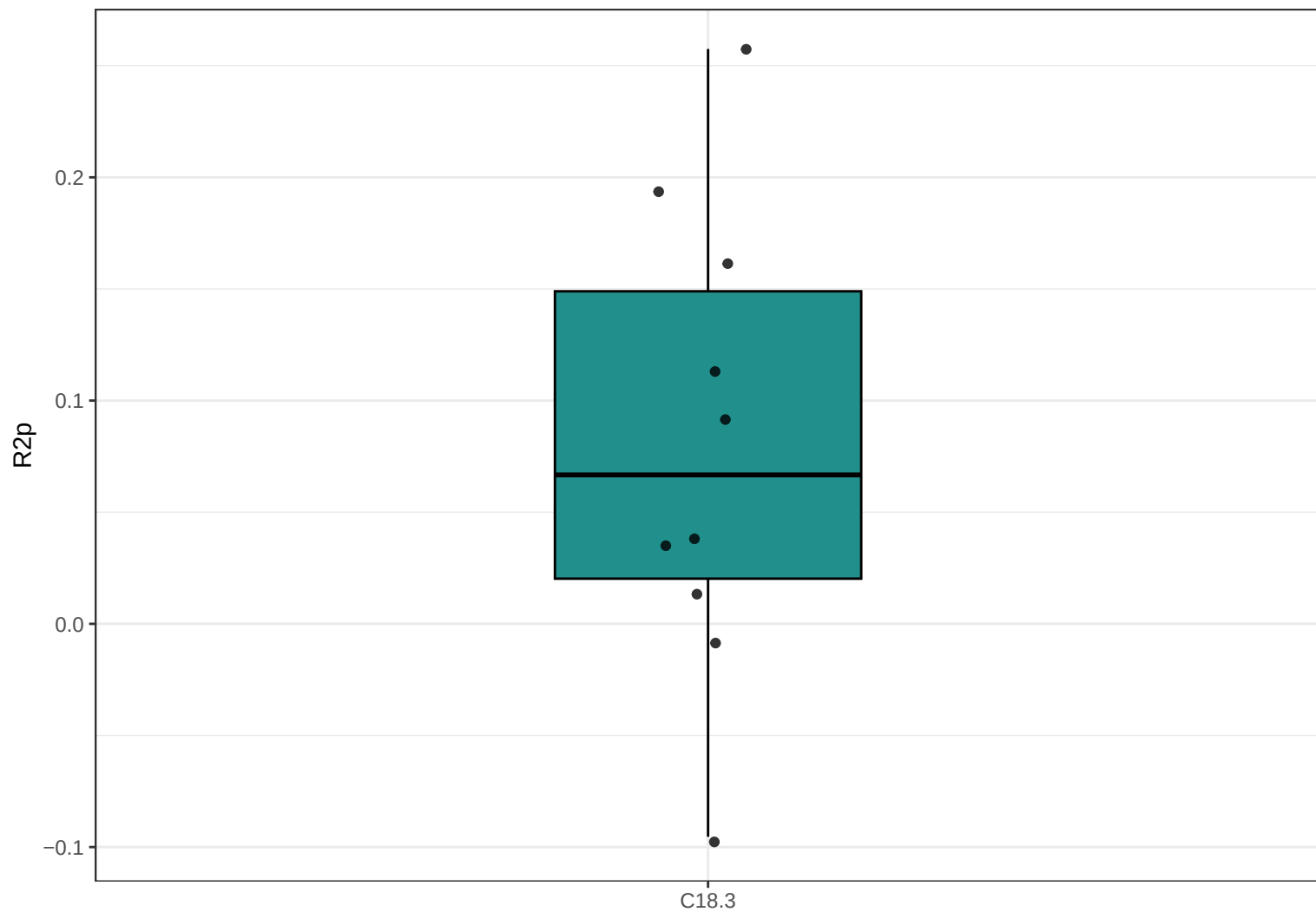
Boxplot R2p (PLS) : C18.3
