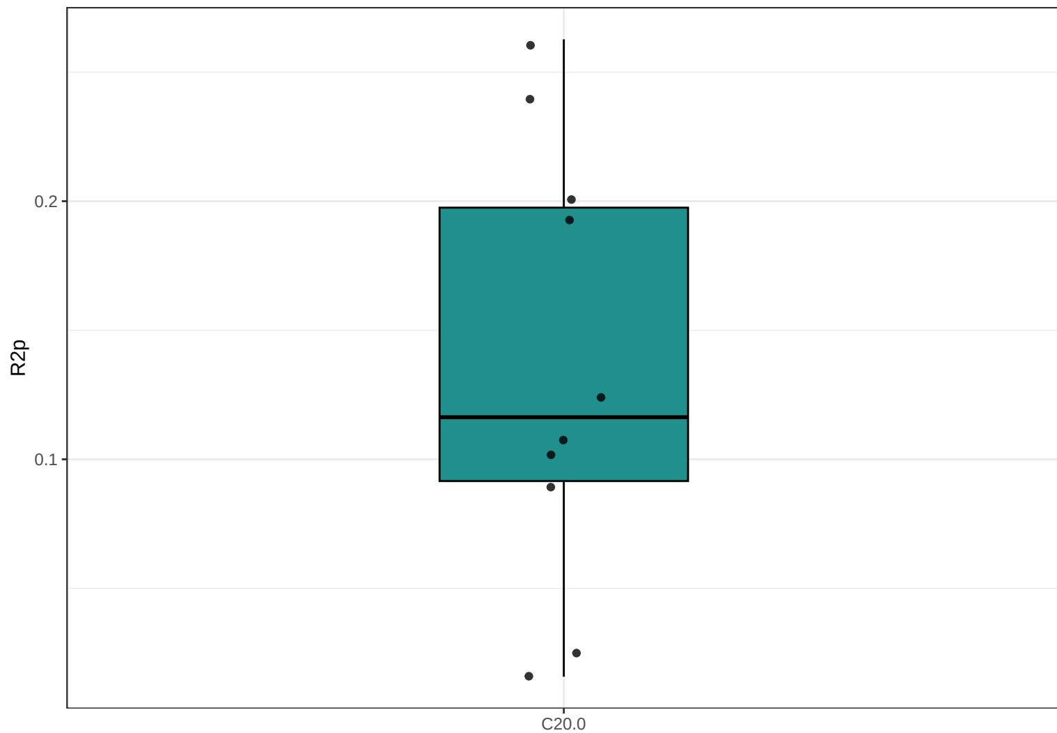
Boxplot R2p (PLS) : C20.0
