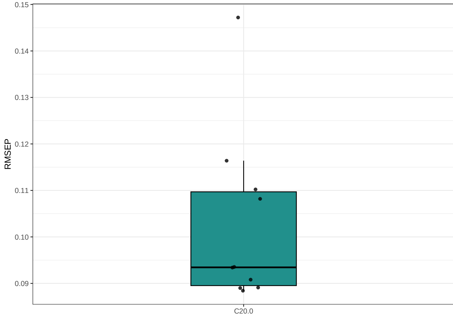
Boxplot RMSEP (PLS) : C20.0
