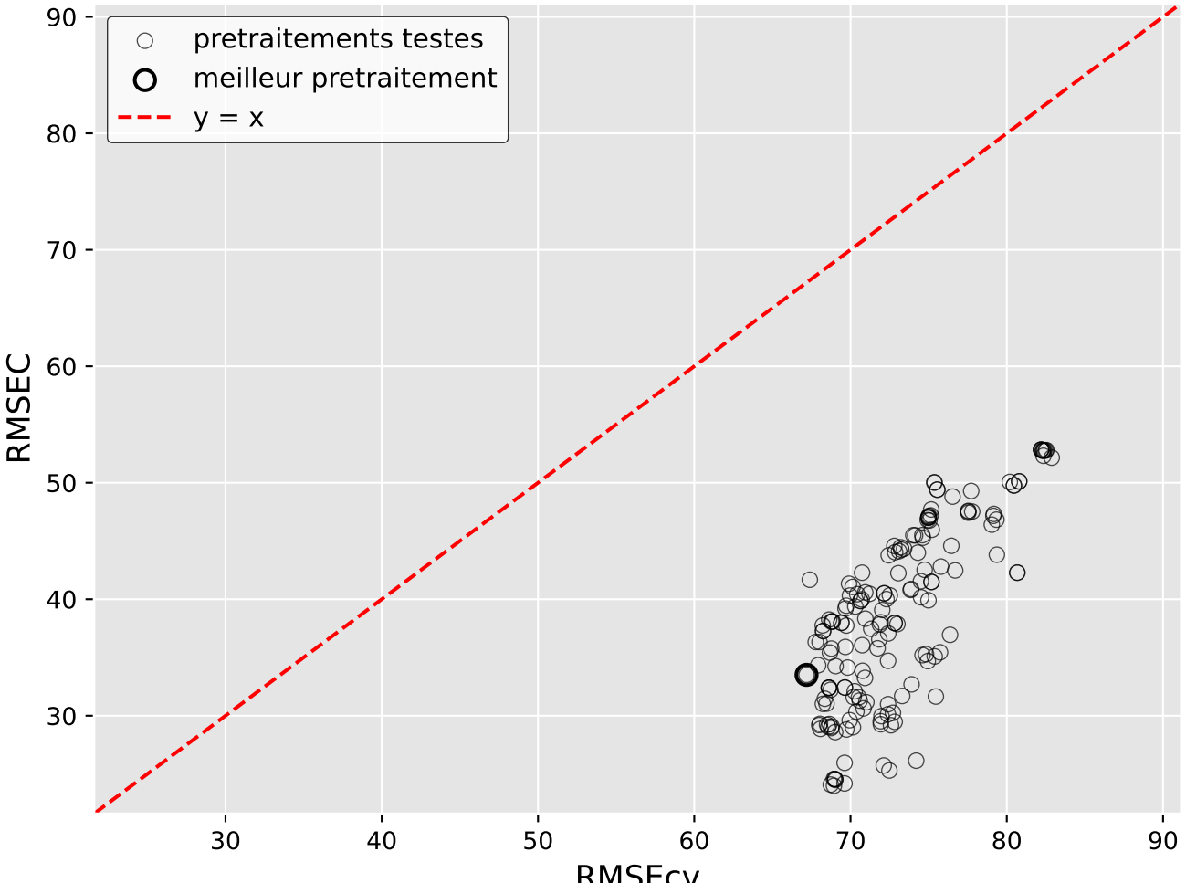
Overfitting pretraitements : aT (Iter 7)
