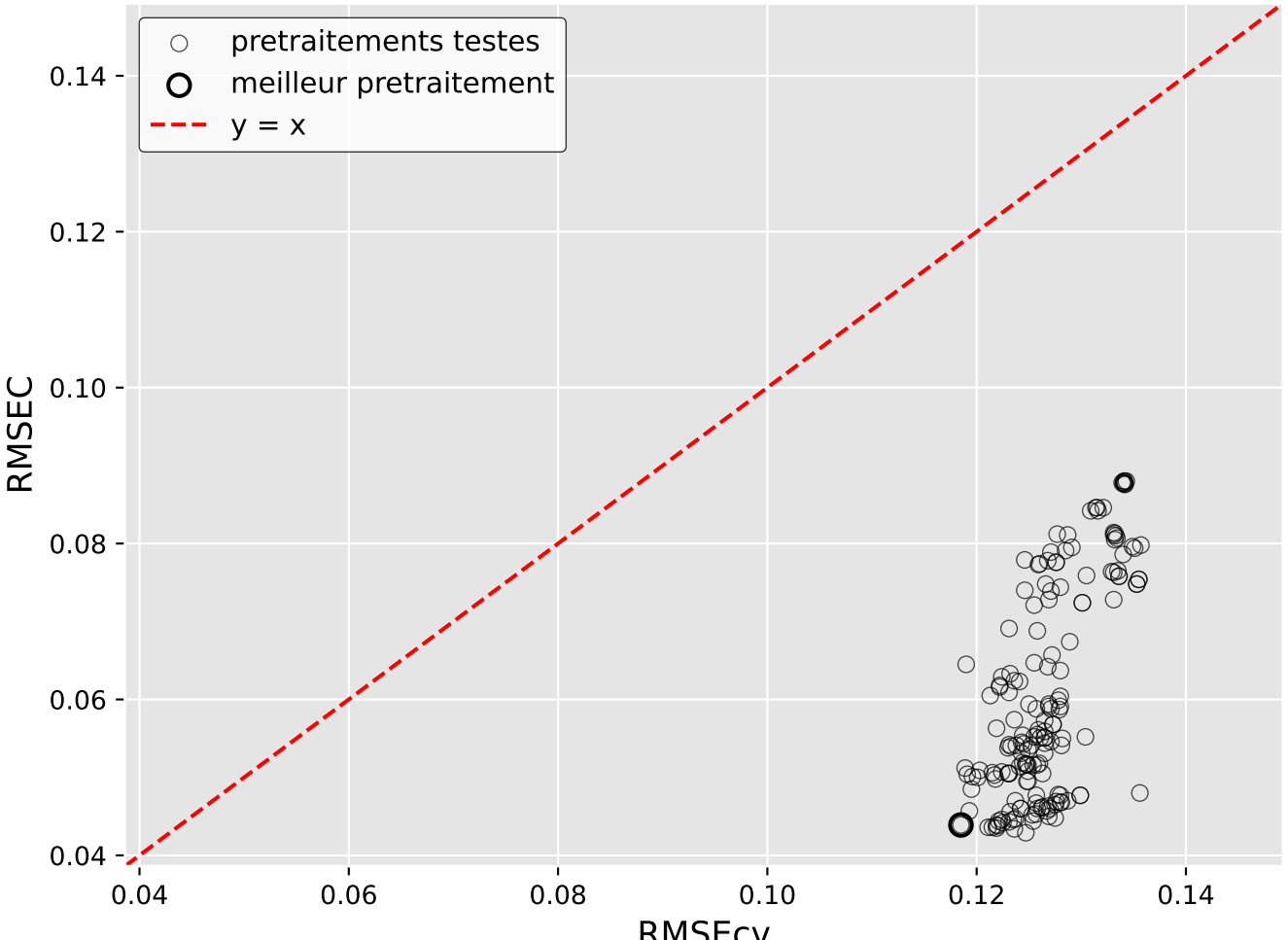
Overfitting pretraitements : ratio.alpha.beta (Iter 1)
