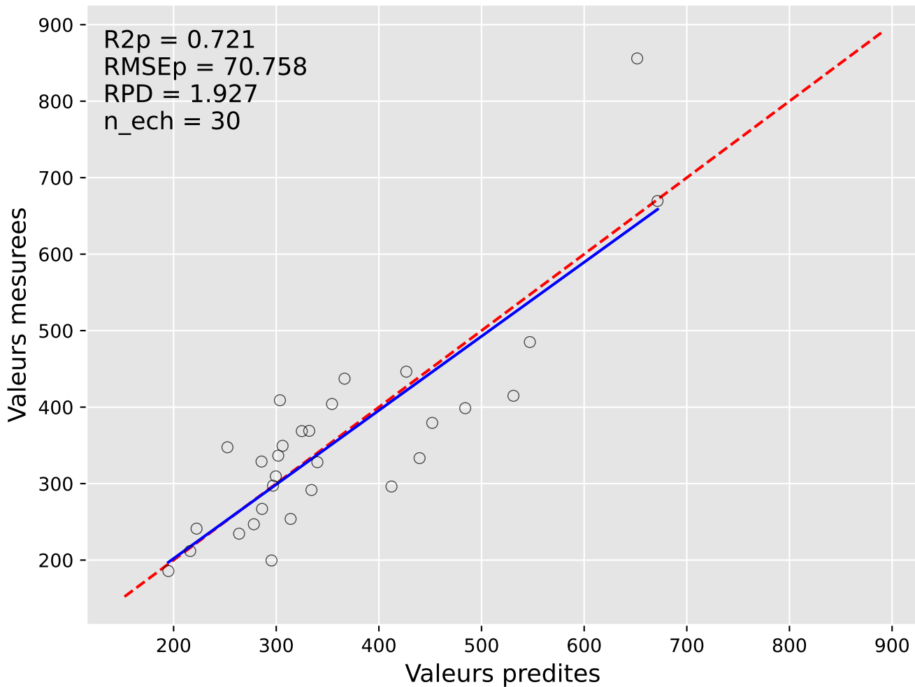
Predictions vs Mesures : trans.alpha.carotene (Iter 4)
