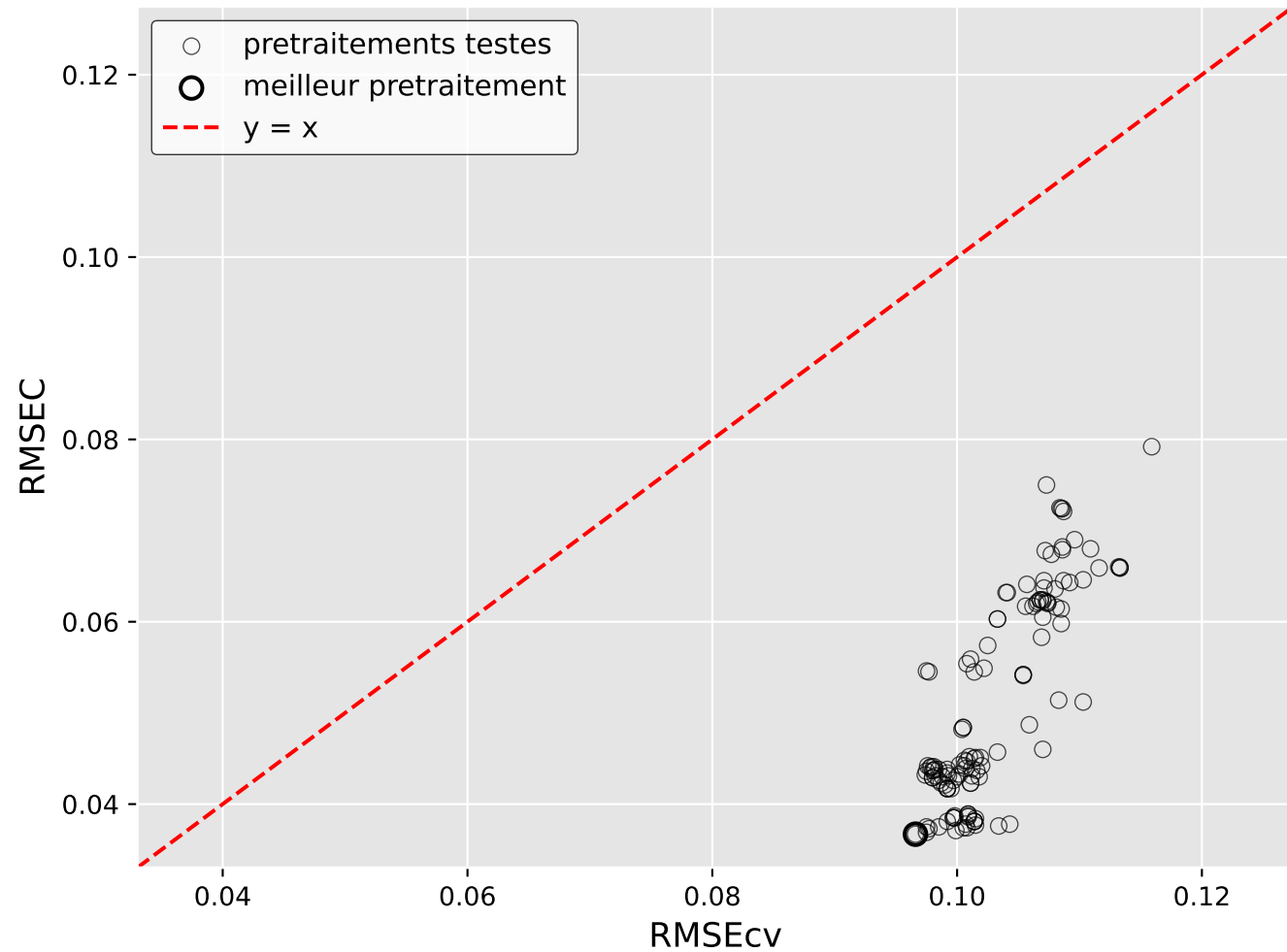
Overfitting pretraitements : C18.3 (Iter 5)
