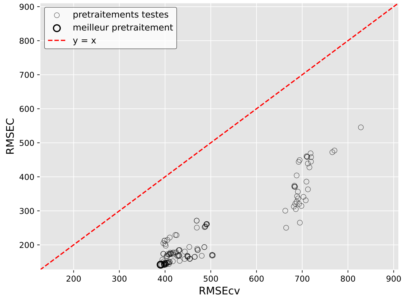
Overfitting pretraitements : total.carotene (lter 10)
