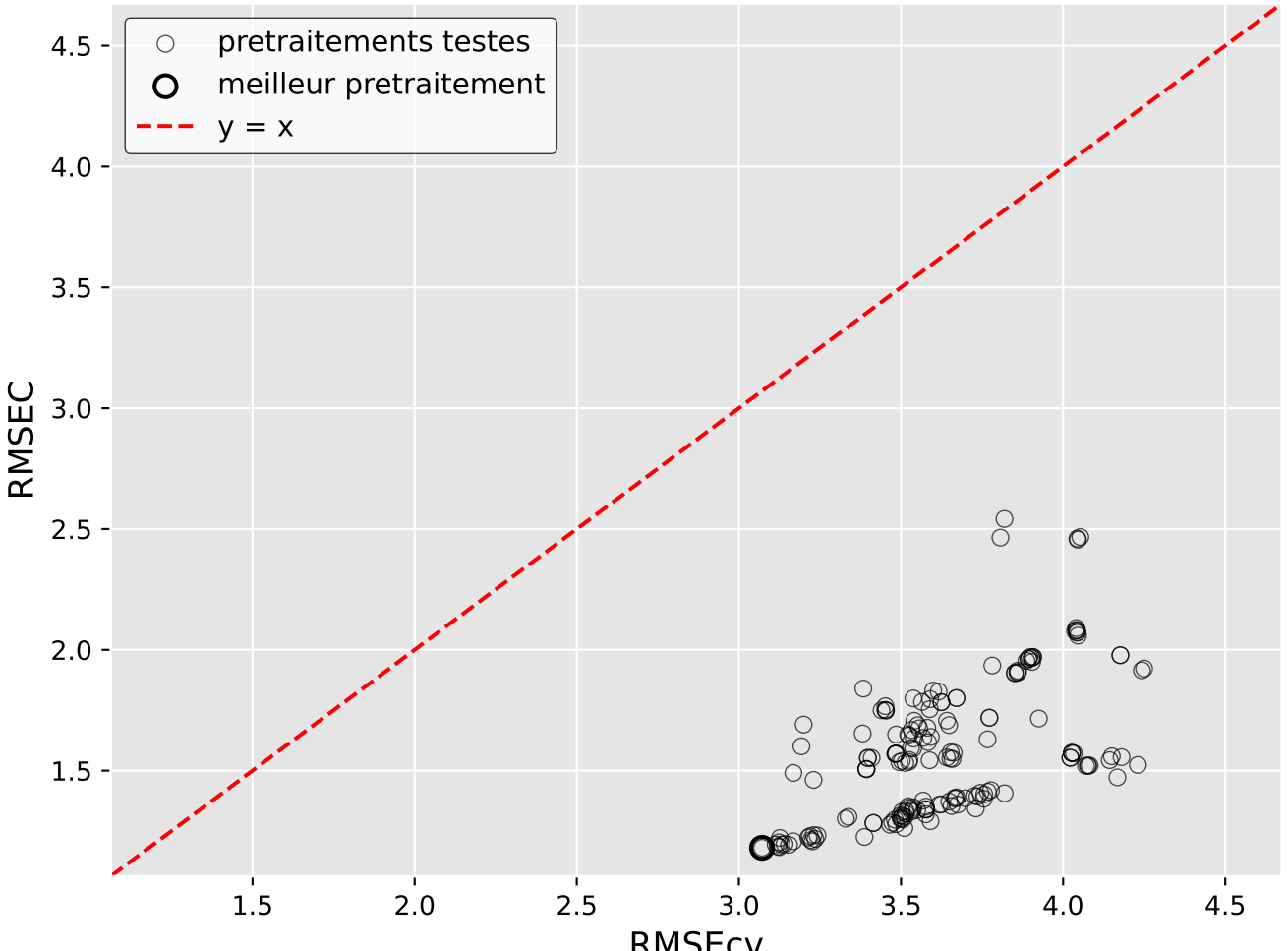
Overfitting pretraitements : tlip.MS (Iter 4)
