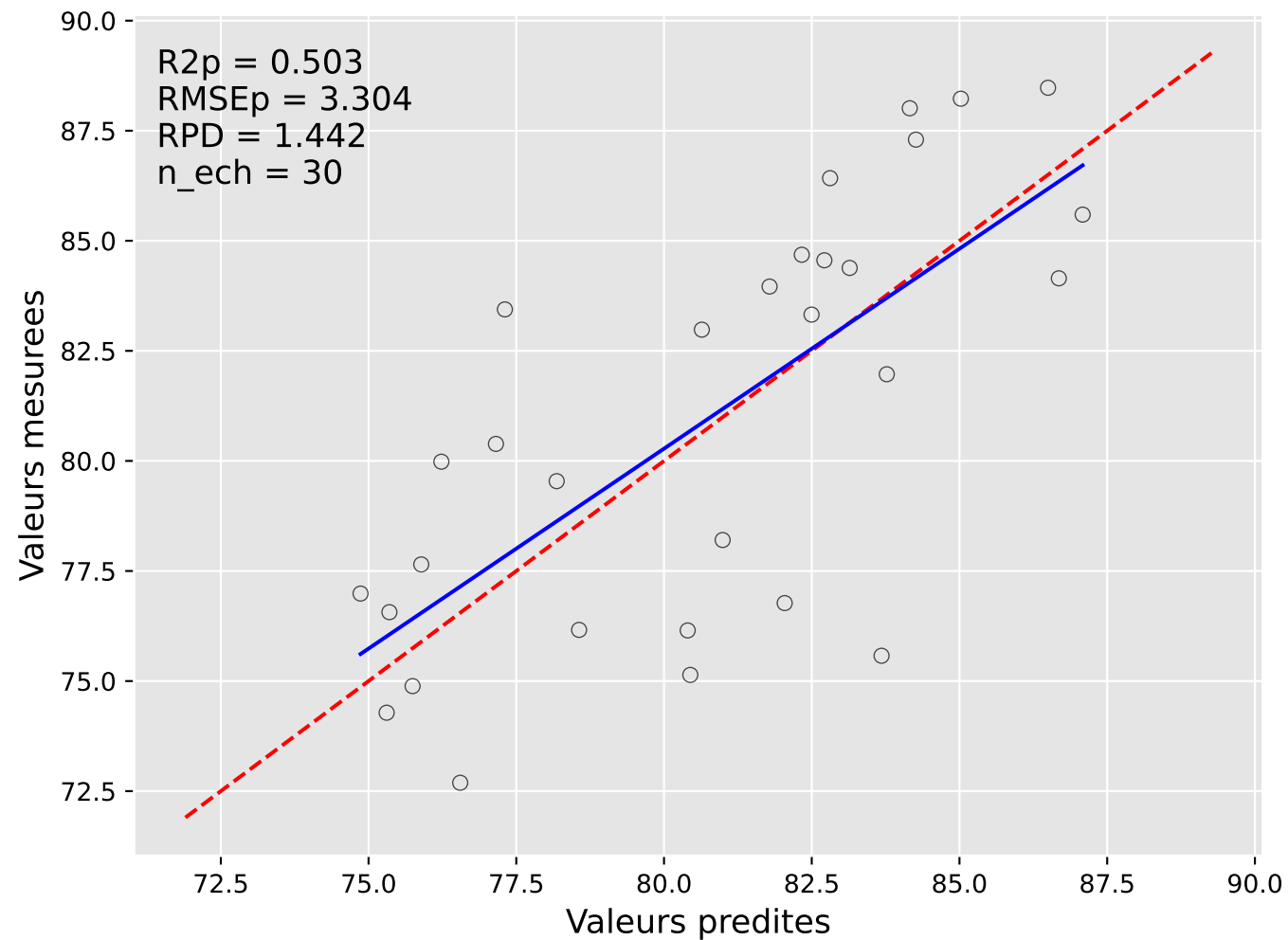
Predictions vs Mesures : tlip.MS (Iter 4)
