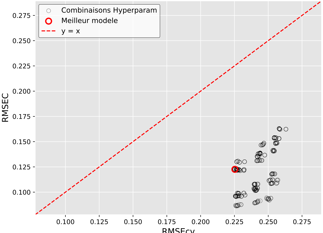
Overfitting Hyperparametres (Iter 8)
