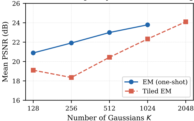
Reconstruction quality on Kodak (24 images)
