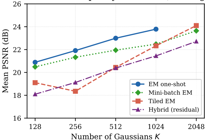
Reconstruction quality on Kodak (24 images)
