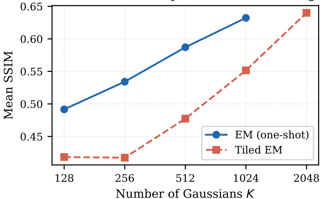
Structural similarity on Kodak (24 images)
