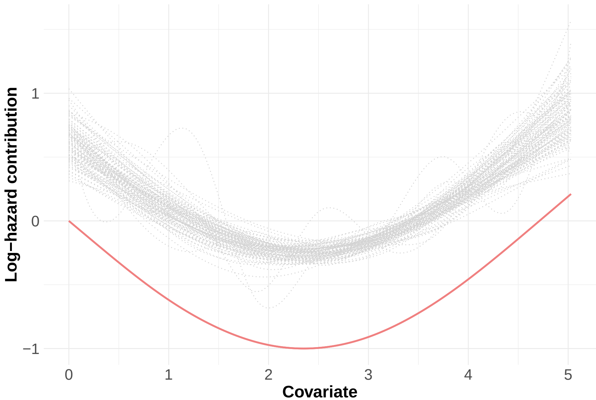
ESTIMATED vs TRUE non-linear effect (Model with SHIFTING)
