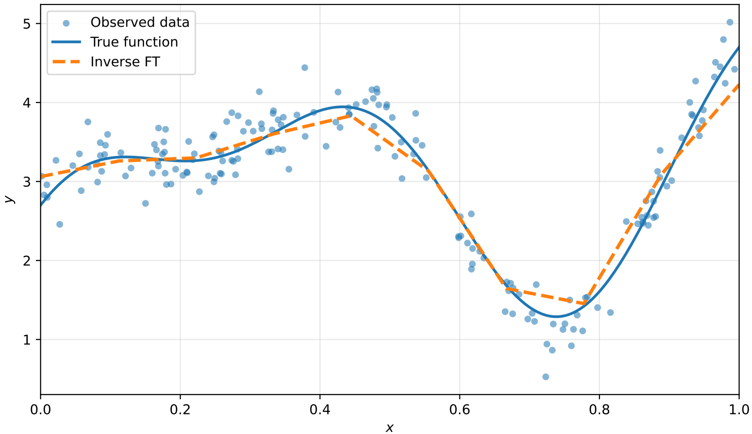
Inverse fuzzy transform: n = 10 fuzzy sets
