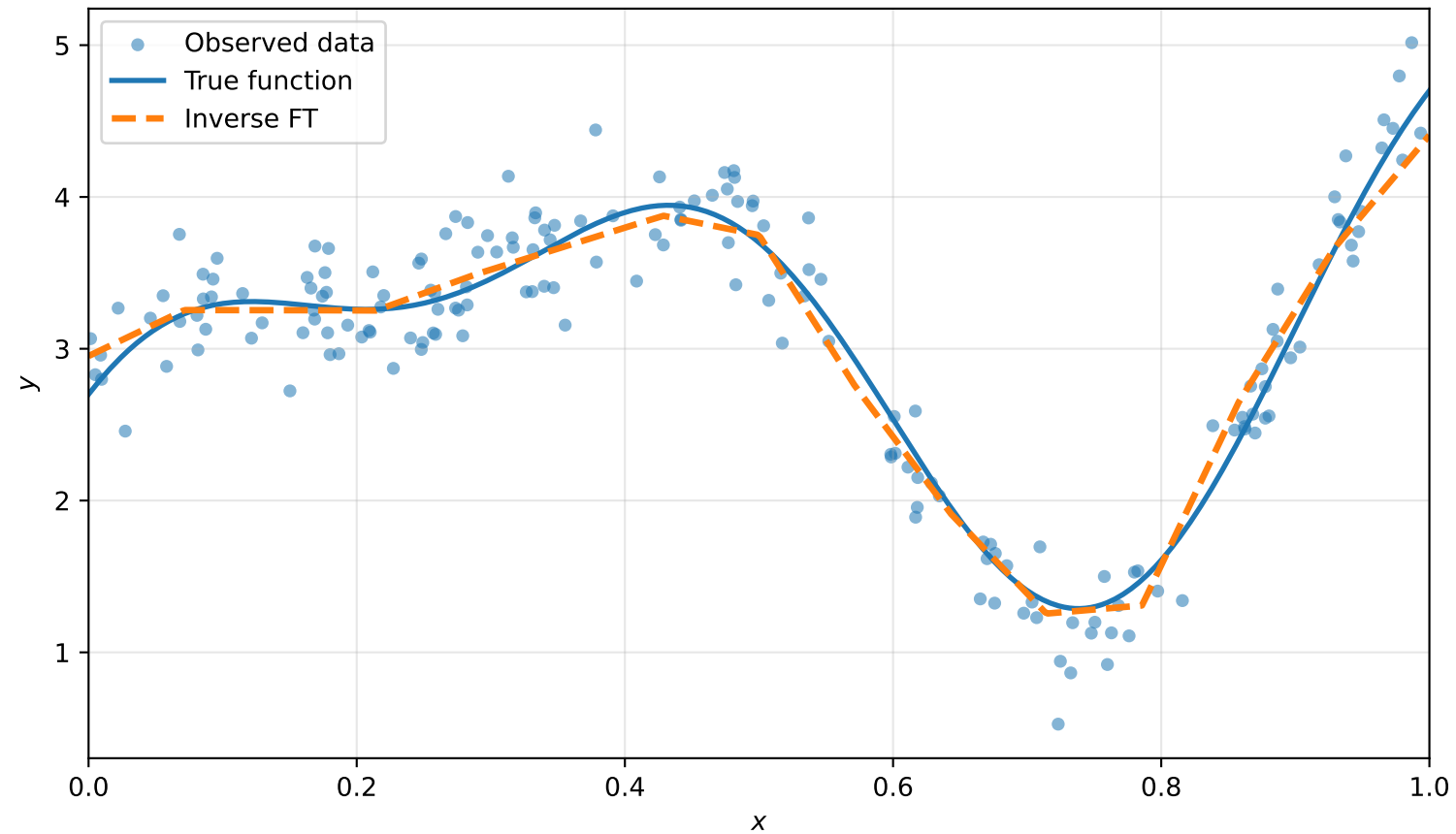
Inverse fuzzy transform: n = 15 fuzzy sets
