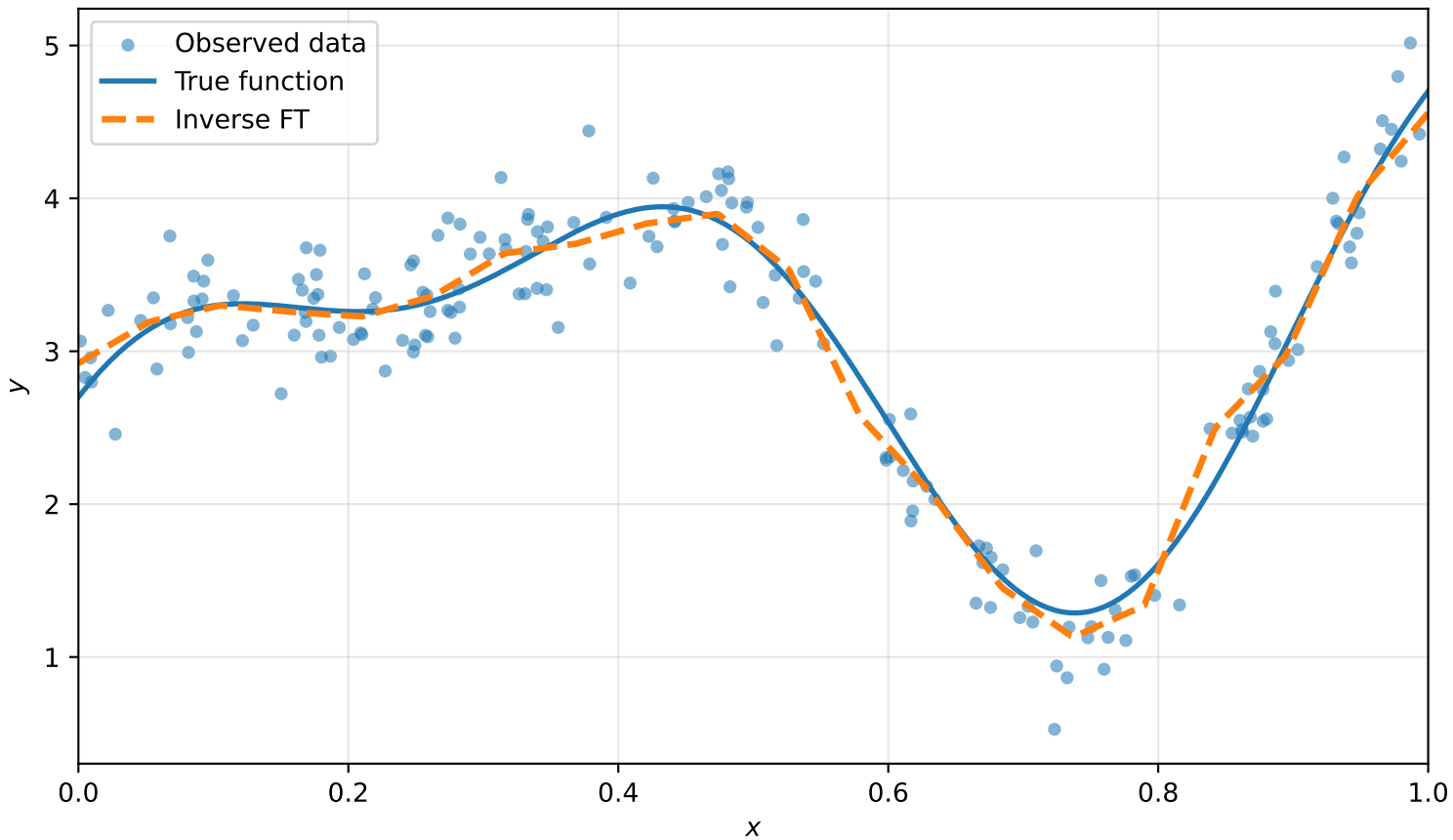
Inverse fuzzy transform: n = 20 fuzzy sets
