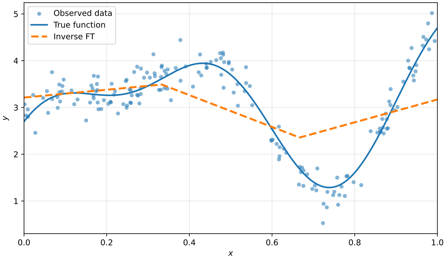
Inverse fuzzy transform: n = 4 fuzzy sets
