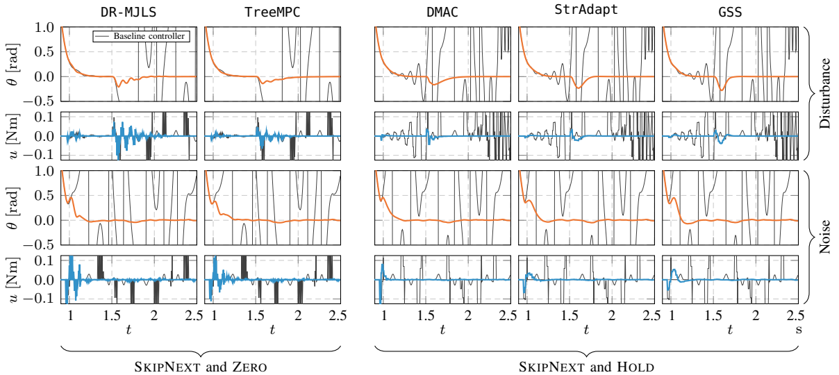
Fig. 3: Furuta pendulum: Trajectories of \theta(t) and u(t) with different disturbance signals and a common sequence (\mu[k]) for some of the applicable controllers, using SKIPNEXT and ZERO (left) or SKIPNEXT and HOLD (right).
