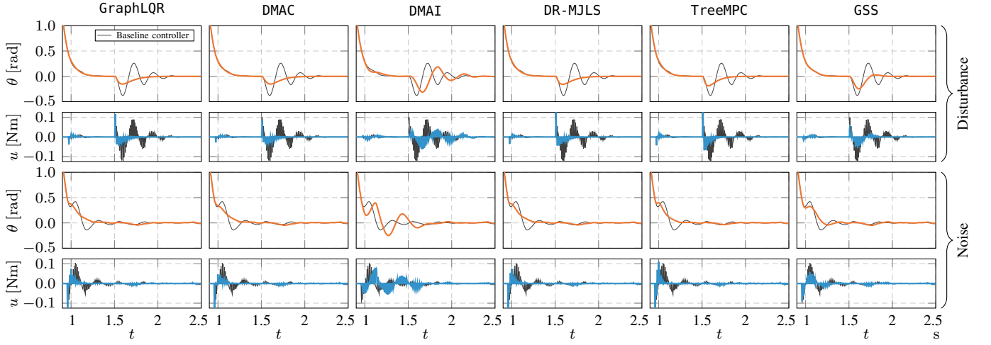
Fig. 1: Furuta pendulum: Trajectories of pendulum angle \theta(t) and system input u(t) with different disturbance signals and a common sequence (\mu[k]) , using KILL and ZERO.
