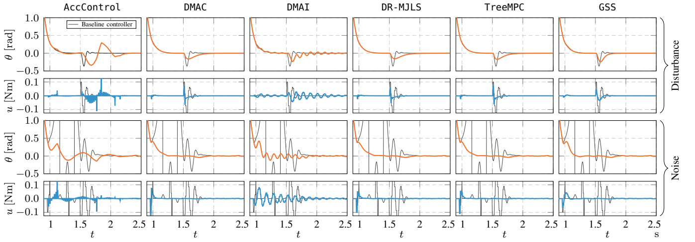
Fig. 2: Furuta pendulum: Trajectories of \theta(t) and u(t) with different disturbance signals and a common sequence (\mu[k]) , using KILL and HOLD.
