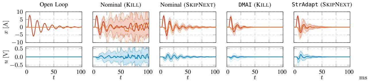
Fig. 6: Electric motor: Trajectories and 0.1–0.9 quantiles of states i_d(t) (—), i_q(t) (—) and inputs u_d(t) (—), u_q(t) (—) controlled by output-feedback at an upper bound of the job response time \bar{t} = 2.5 T . The trajectories of \omega_{el}(t) are omitted.
