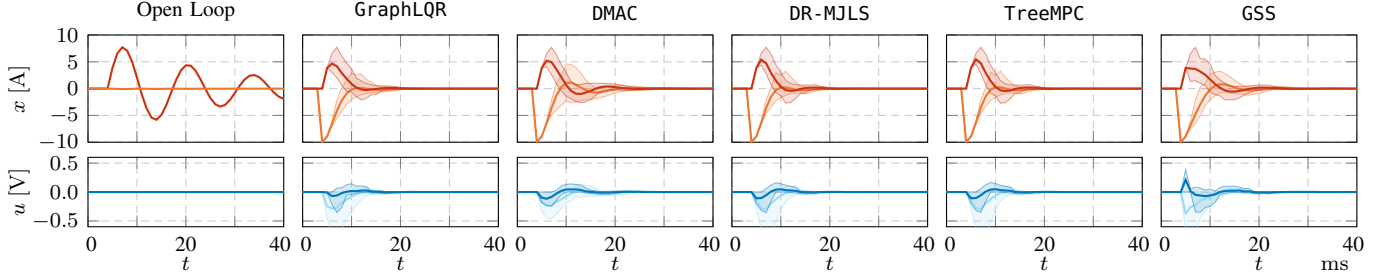
Fig. 4: Electric motor: State trajectories i_d(t) (—), i_q(t) (—) and inputs u_d(t) (—), u_q(t) (—) with offset disturbance, using KILL and ZERO. The 0.1–0.9 quantiles are shown with opacity. The trajectories of \omega_{el}(t) are omitted.
