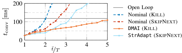
Fig. 7: Electric motor: Convergence times t_{\text{conv}} against different upper bounds of the job response times \bar{t} .
