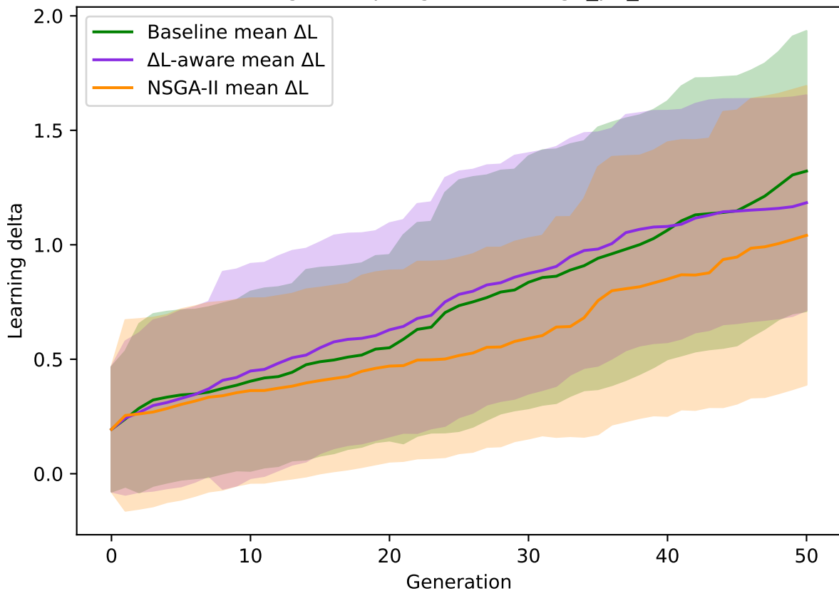
Mean learning delta per generation (ga_p2_seeds10-10)
