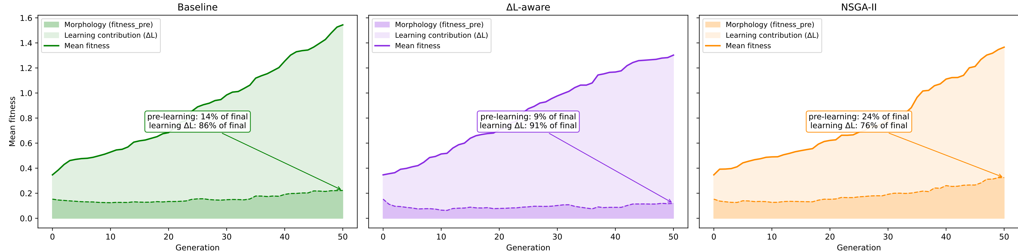
Mean fitness decomposition: morphology vs learning (ga_p2_seeds10-10)
