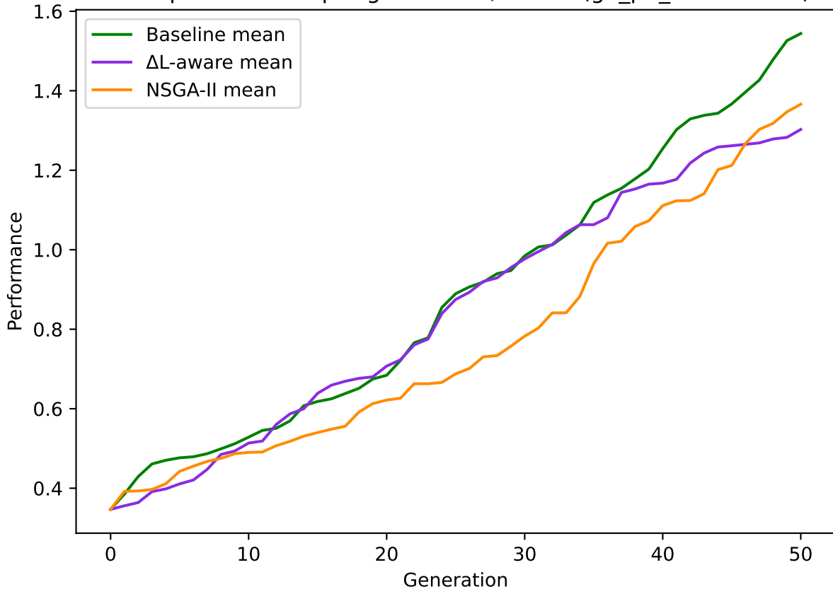
Mean performance per generation, no std (ga_p2_seeds10-10)
