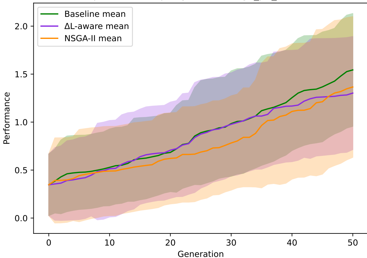
Mean performance per generation (ga_p2_seeds10-10)
