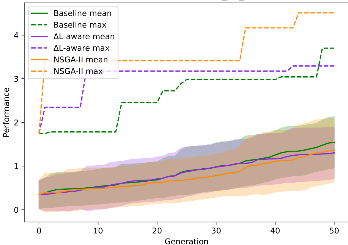
Performance per generation (ga_p2_seeds10-10)
