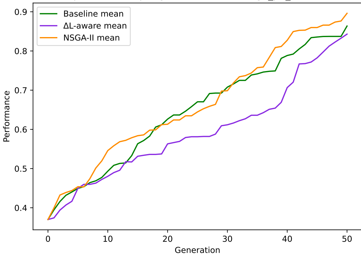
Mean performance per generation, no std (ga_p2_seeds12-12)
