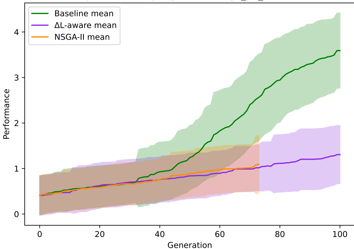
Mean performance per generation (ga_p2_seeds15-15)
