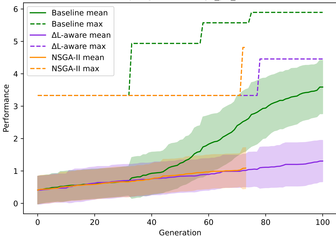
Performance per generation (ga_p2_seeds15-15)
