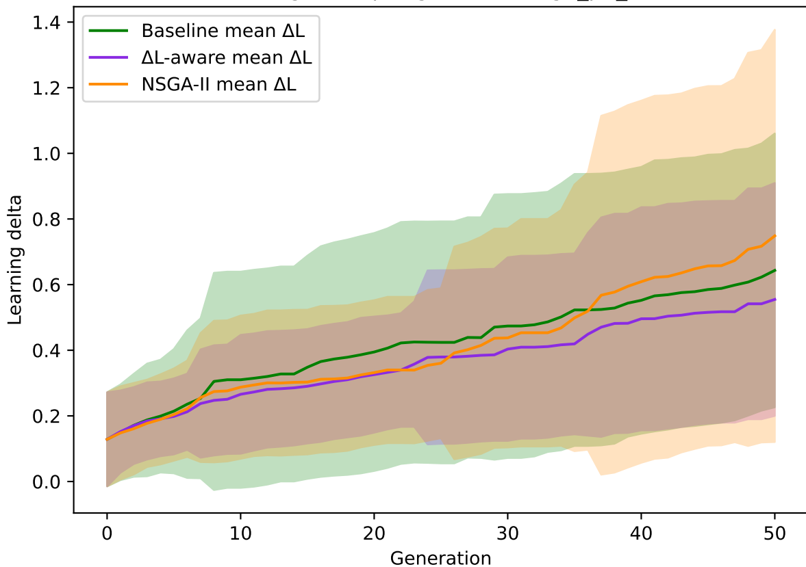
Mean learning delta per generation (ga_p2_seeds7-7)
