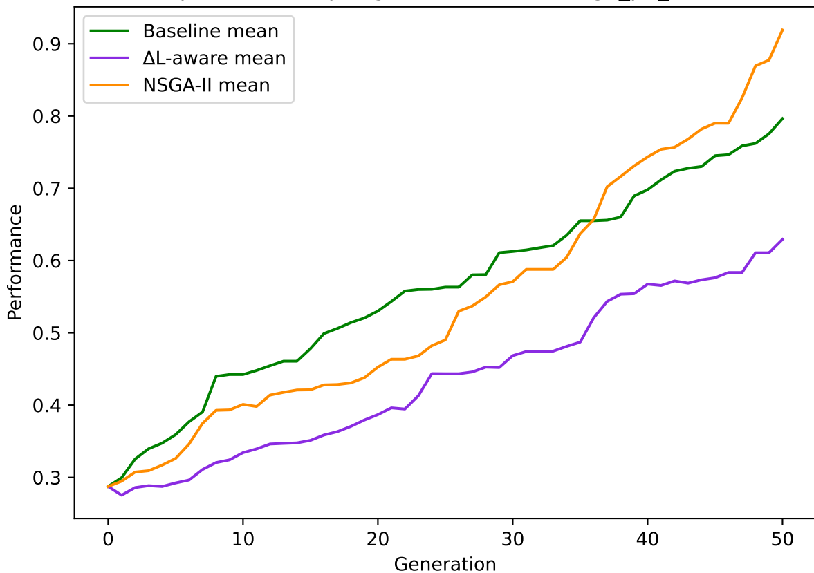
Mean performance per generation, no std (ga_p2_seeds7-7)
